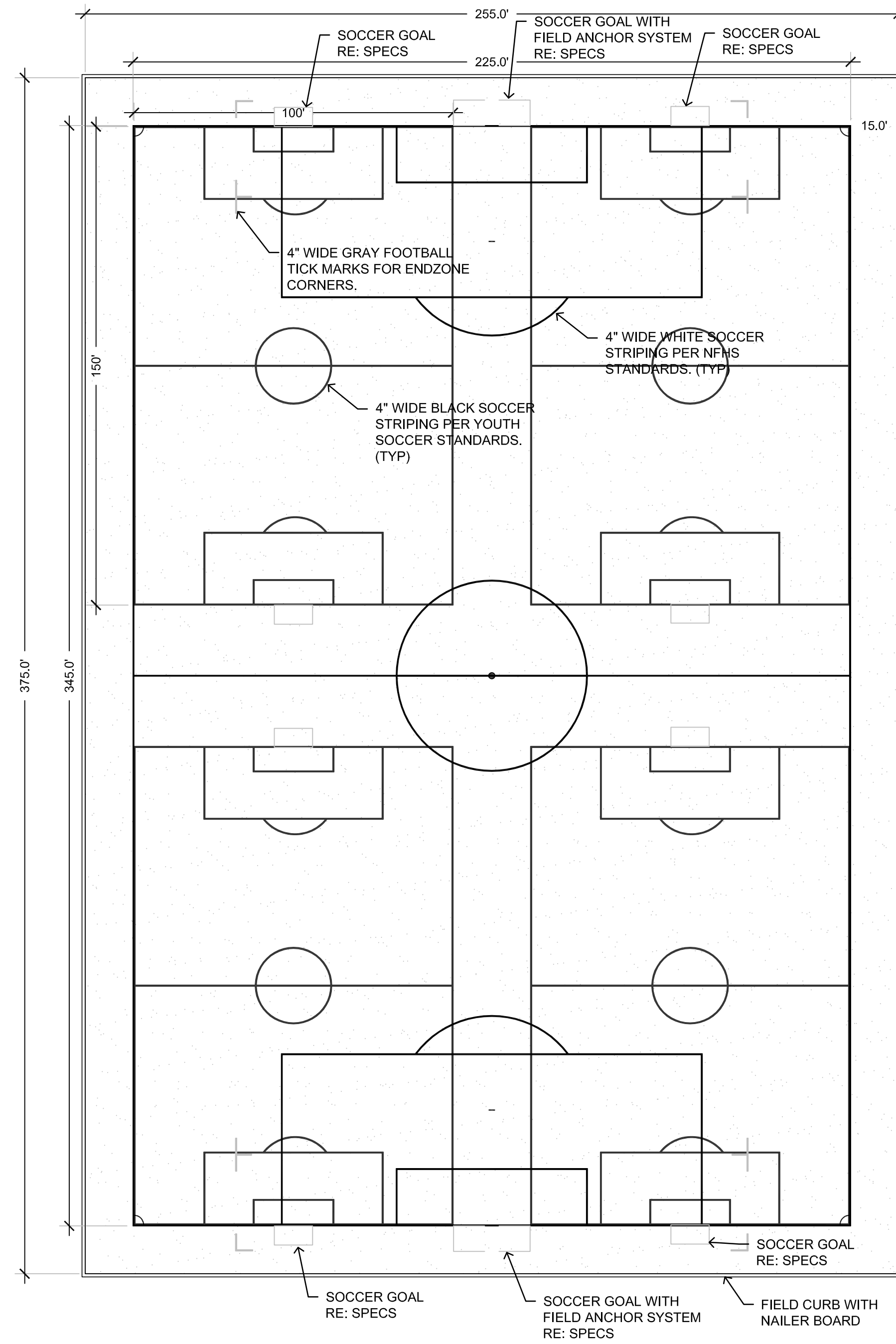
LAYOUT PLAN
