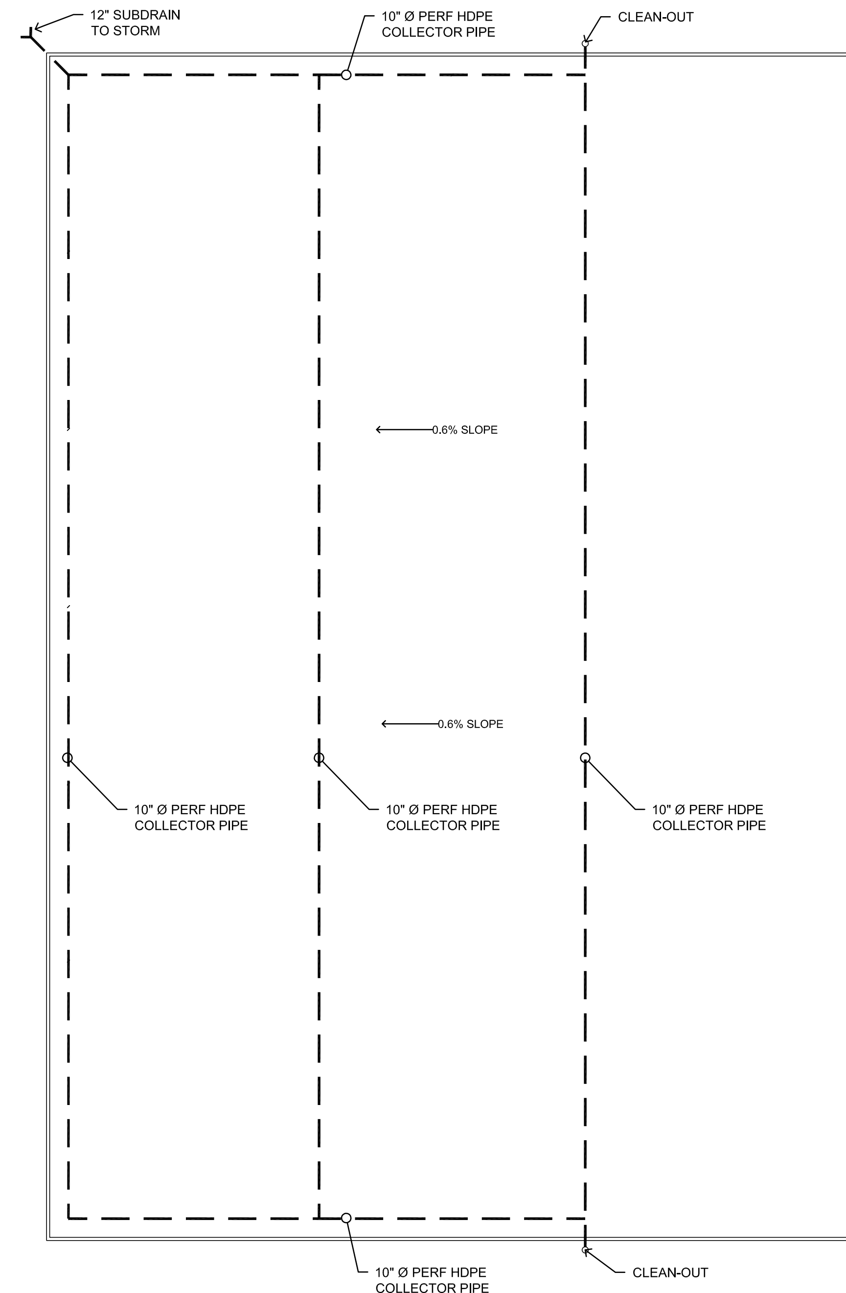
DRAINAGE PLAN
