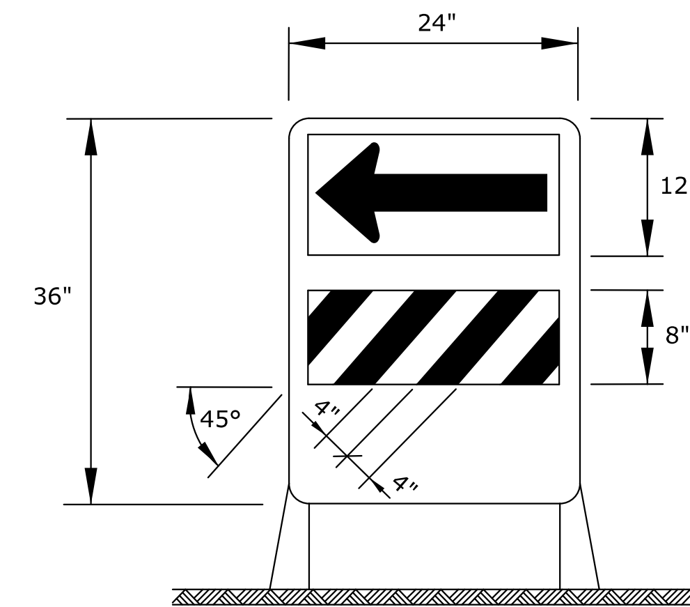
DIRECTION INDICATOR BARRICADE The stripes shall slope downward in the direction traffic is to pass. The direction indicator barricade shall be used in series to direct the motorist into the intended lane of travel.
