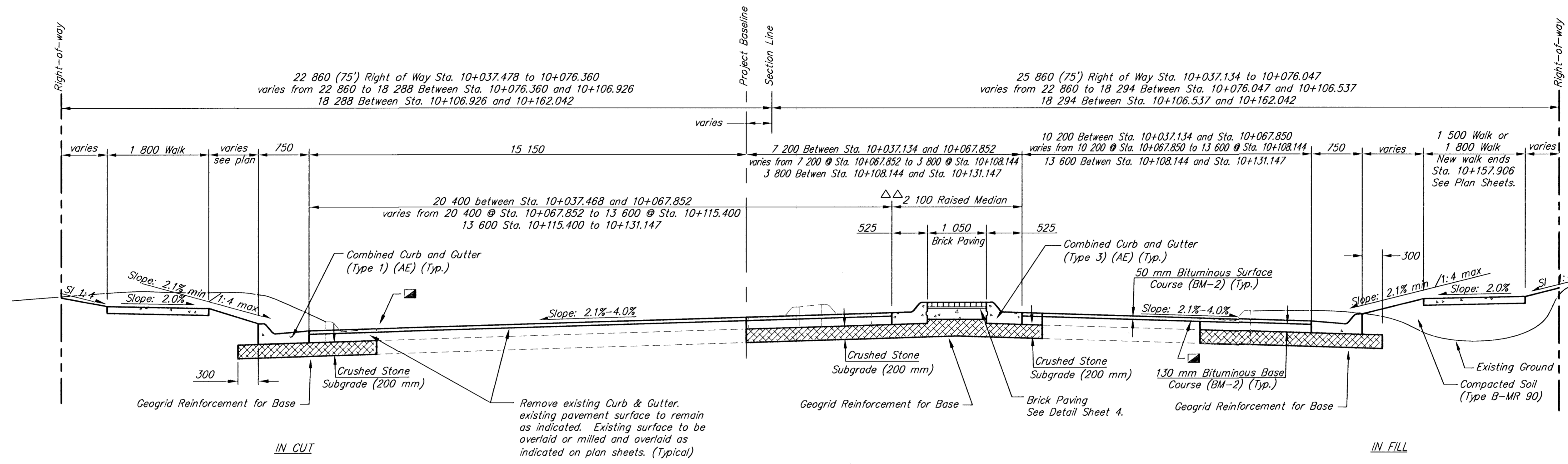
TYPICAL SECTION 10+037.134 TO 10+162.042
