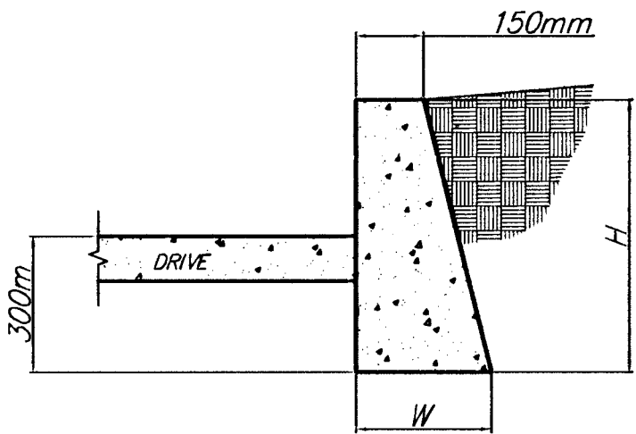
GRAVITY WALL DETAIL (CONCRETE)
