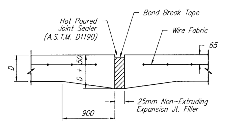
EXPANSION JOINT
