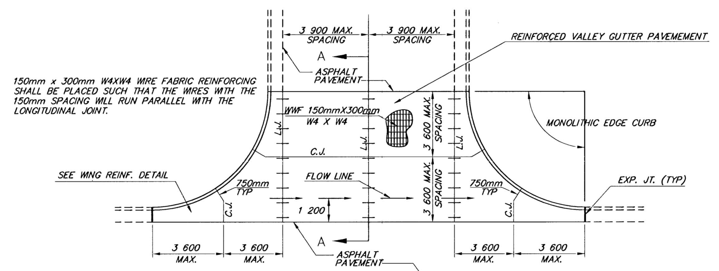
PLAN
