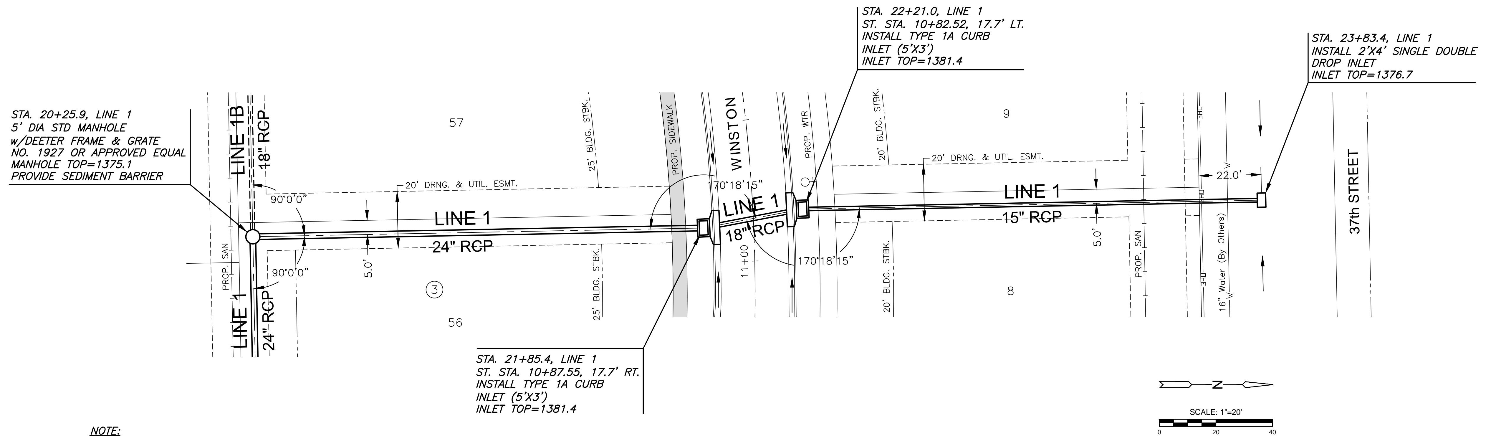
PLAN SWS LINE 1 (CONT.) PROFILE SWS LINE 1 (CONT.)
