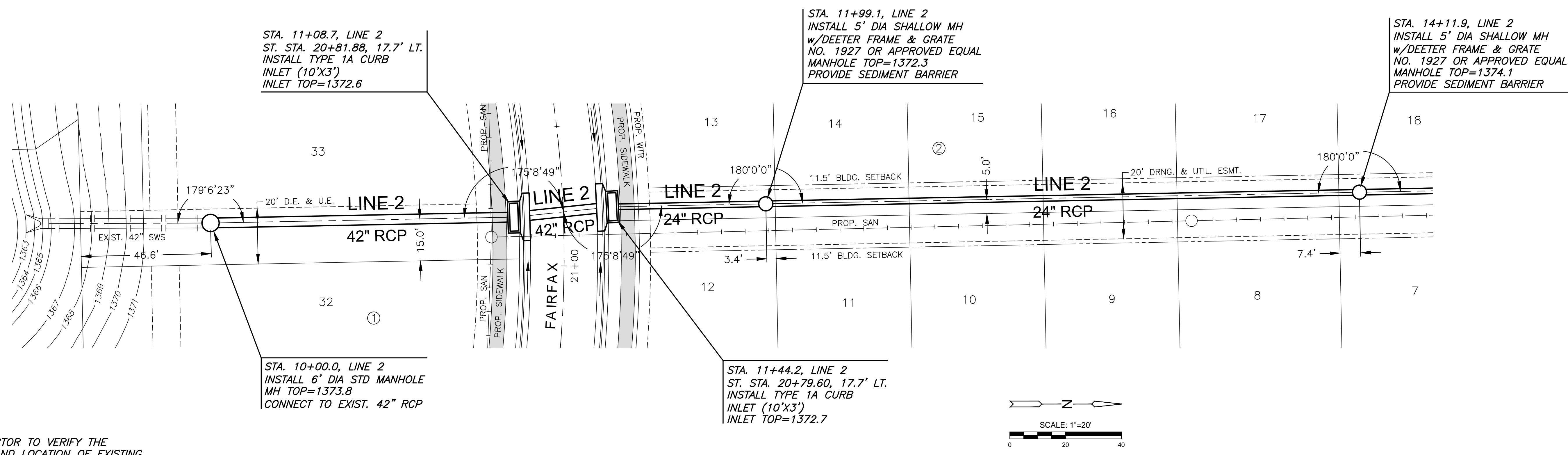
PLAN SWS LINE 2 PROFILE SWS LINE 2
