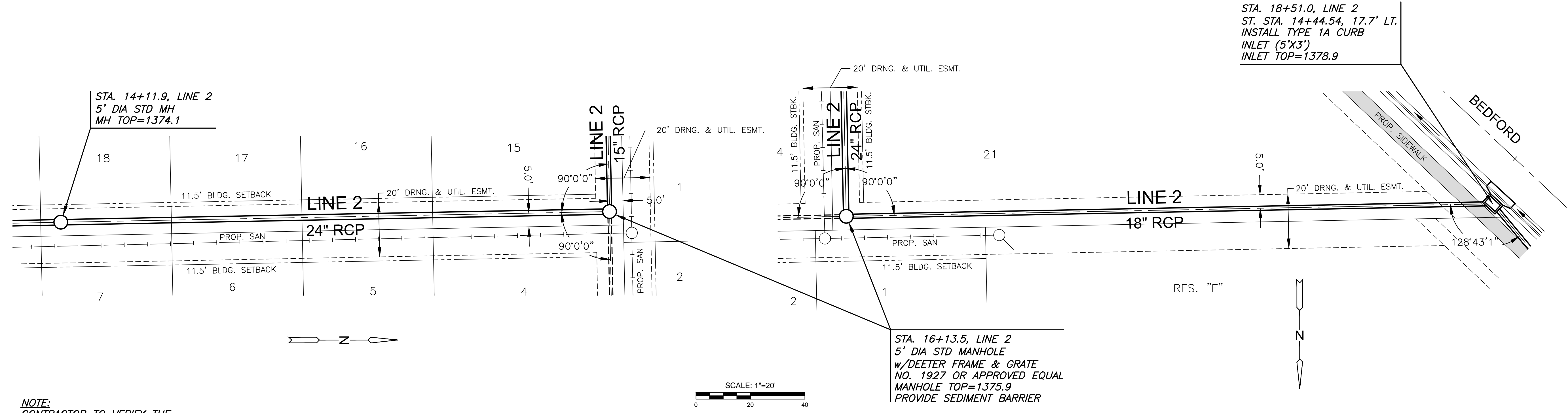
PLAN SWS LINE 2 (CONT.) PROFILE SWS LINE 2 (CONT.)
