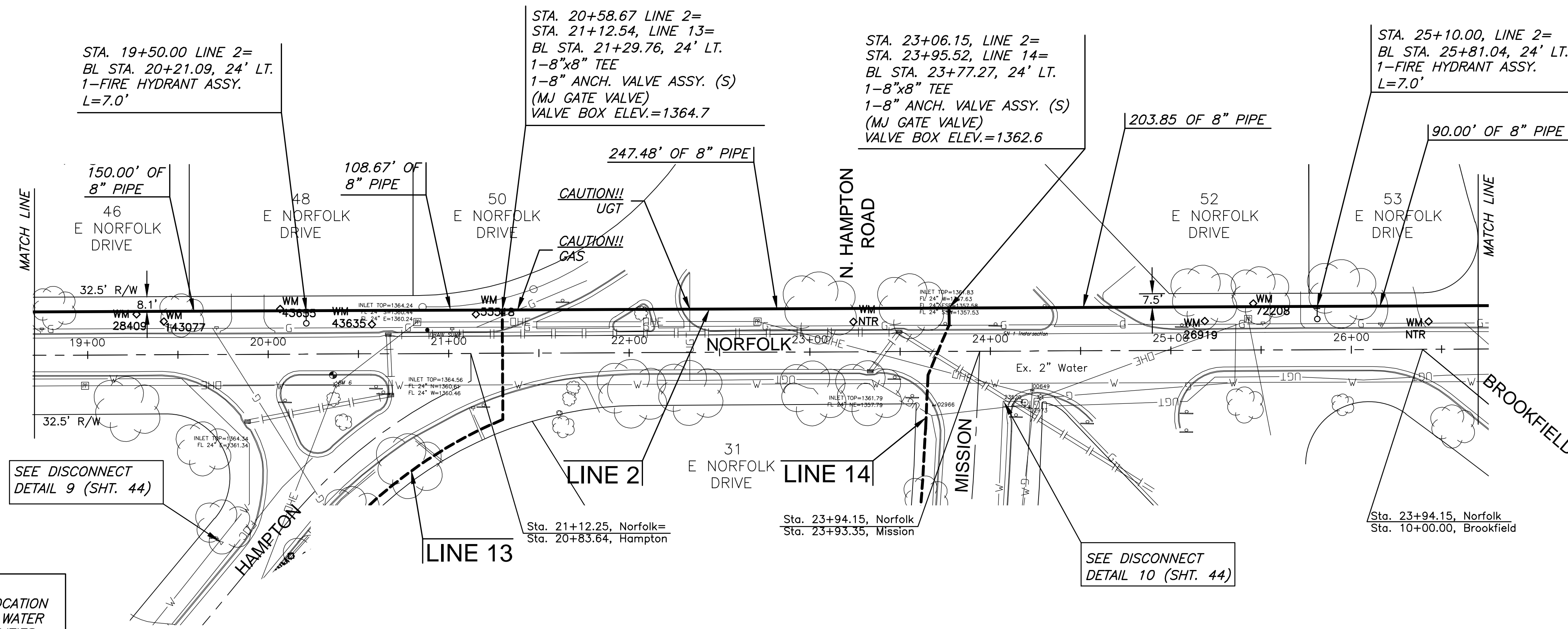
PLAN LINE 2 PROFILE LINE 2
