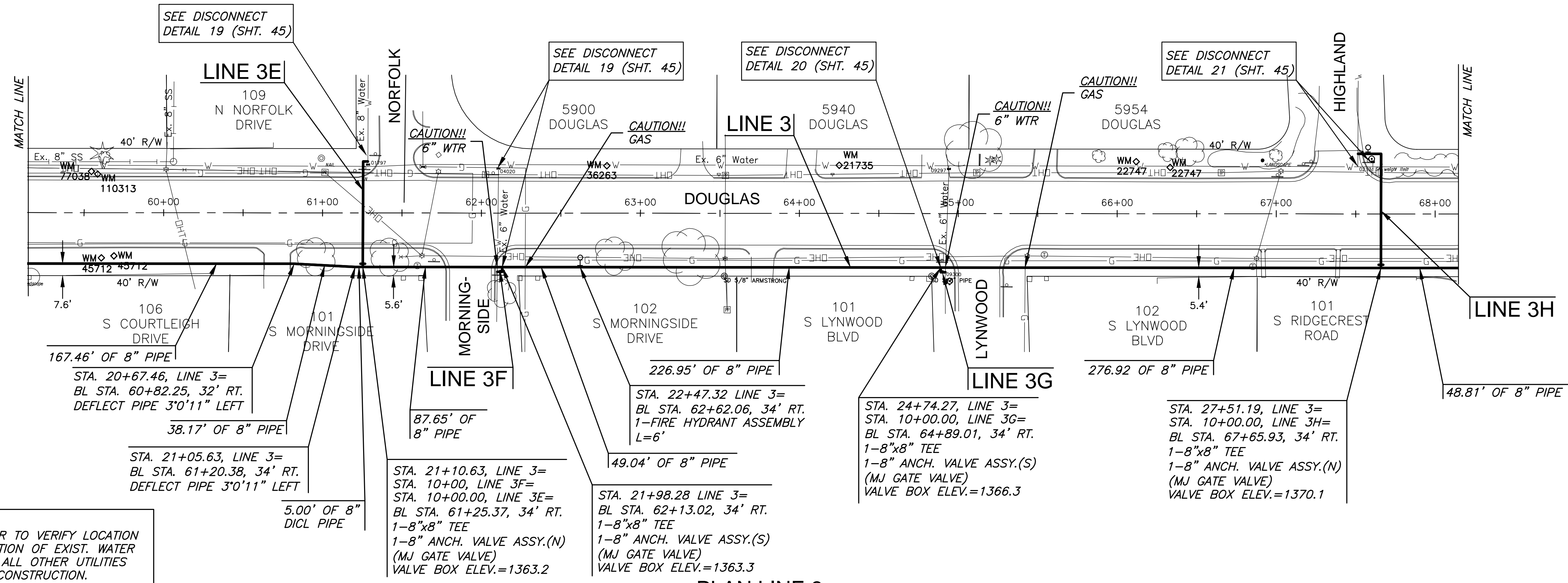
PLAN LINE 3 PROFILE LINE 3
