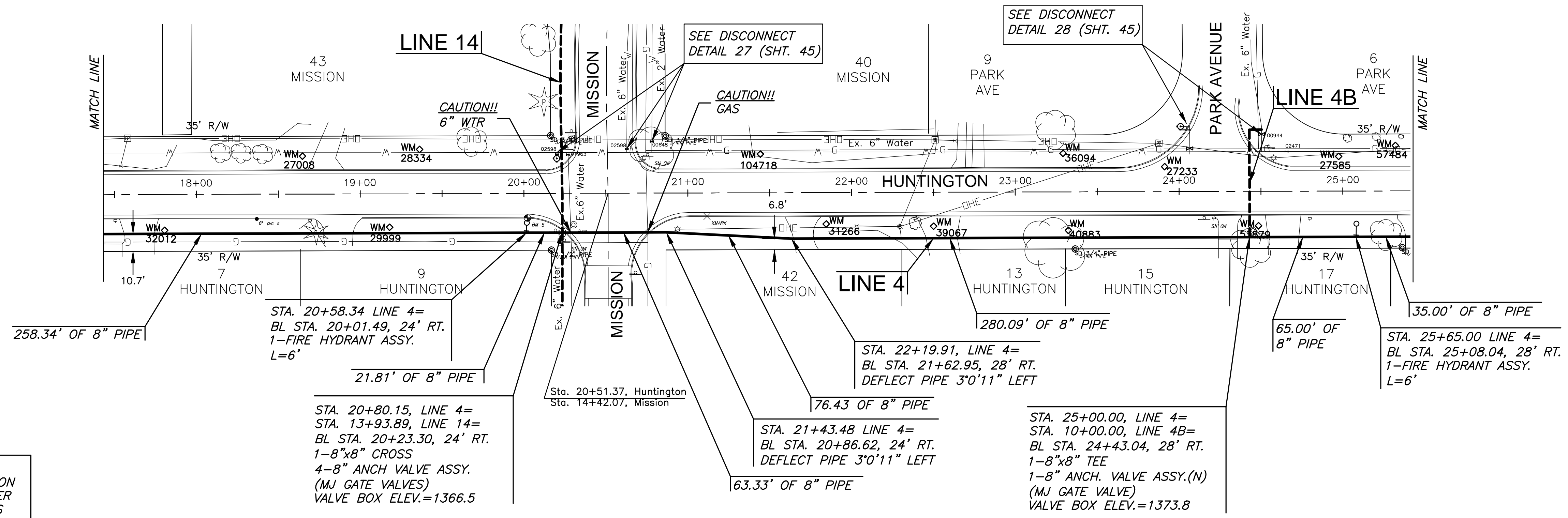
PLAN LINE 4 PROFILE LINE 4
