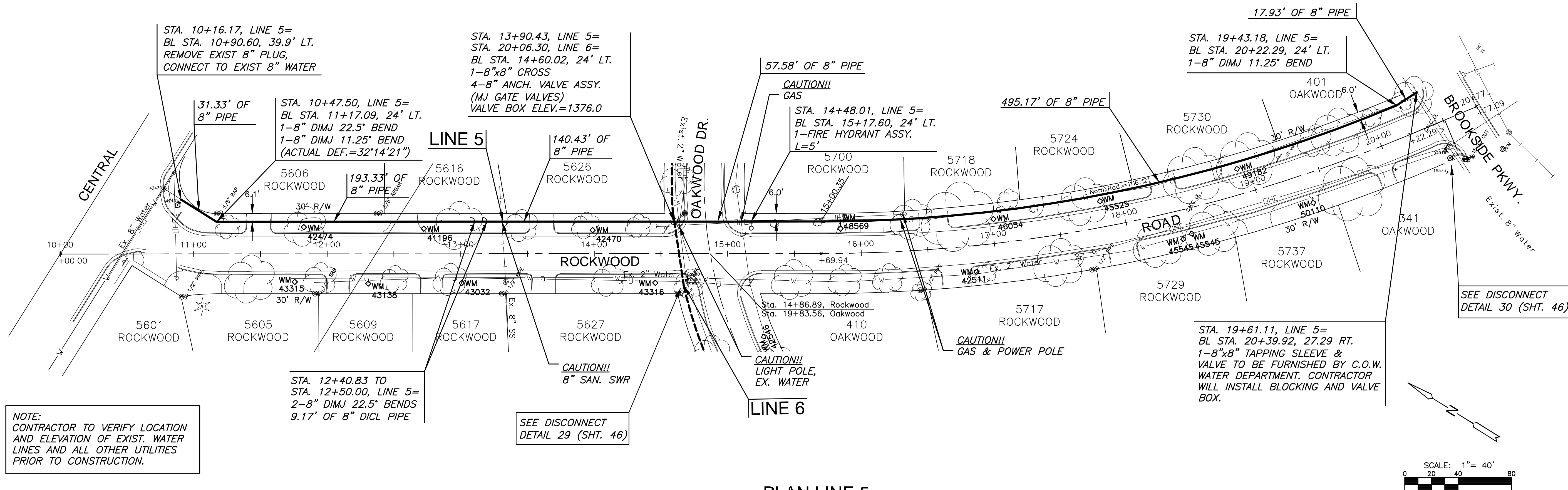
PLAN LINE 5 PROFILE LINE 5
