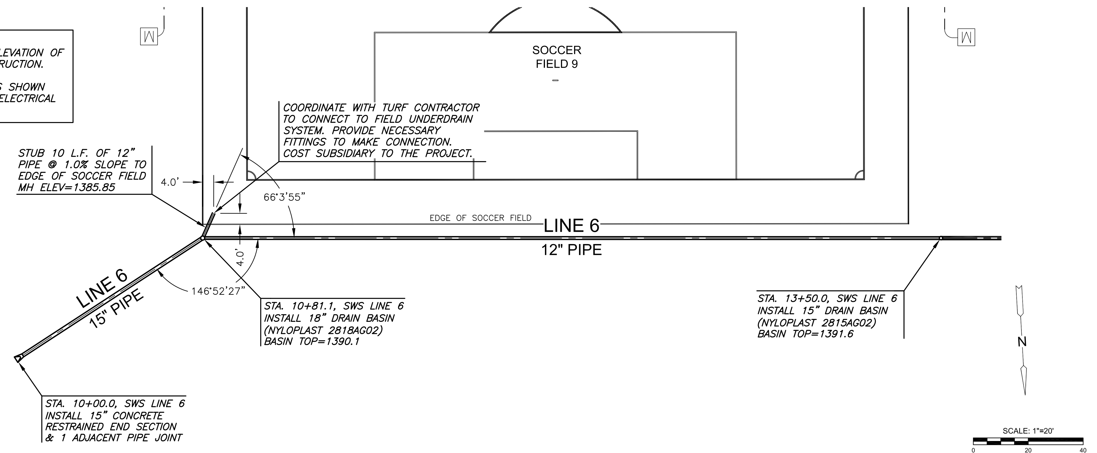
PLAN LINE 6 PROFILE LINE 6
