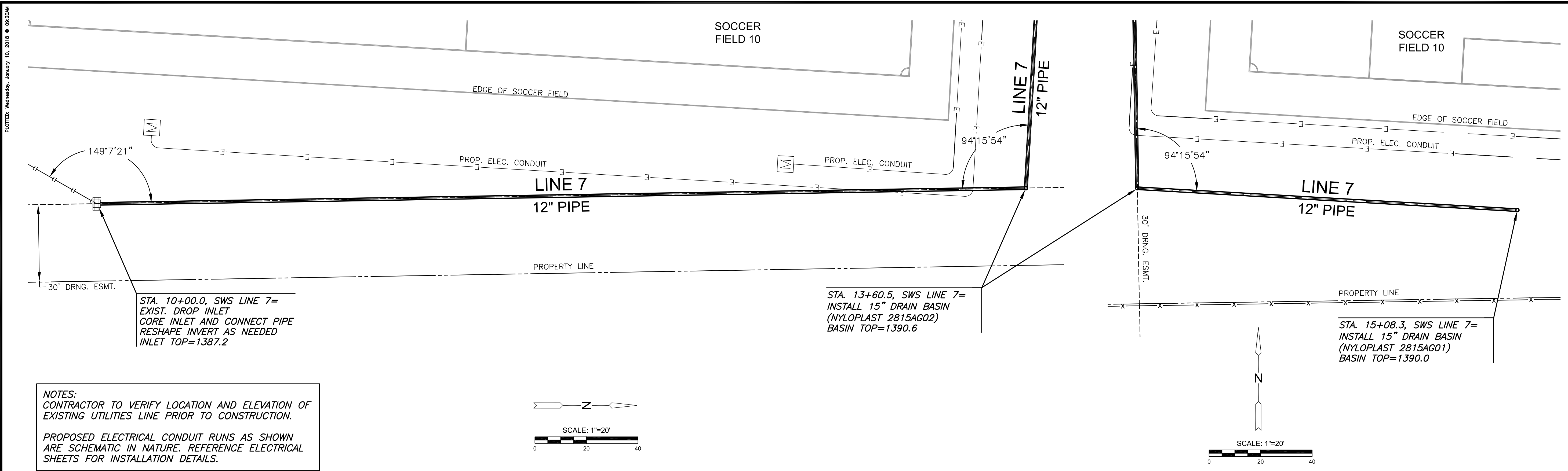
PLAN SWS LINE 7 PROFILE SWS LINE 7
