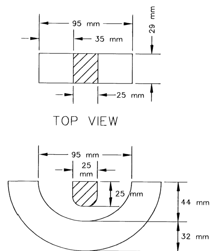
SECTION VIEW
