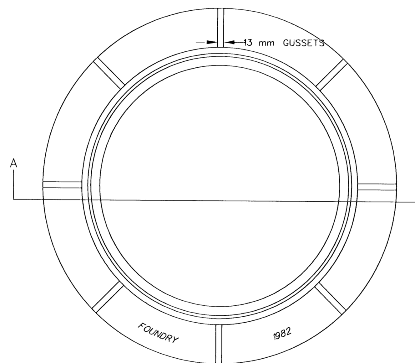
TOP VIEW
