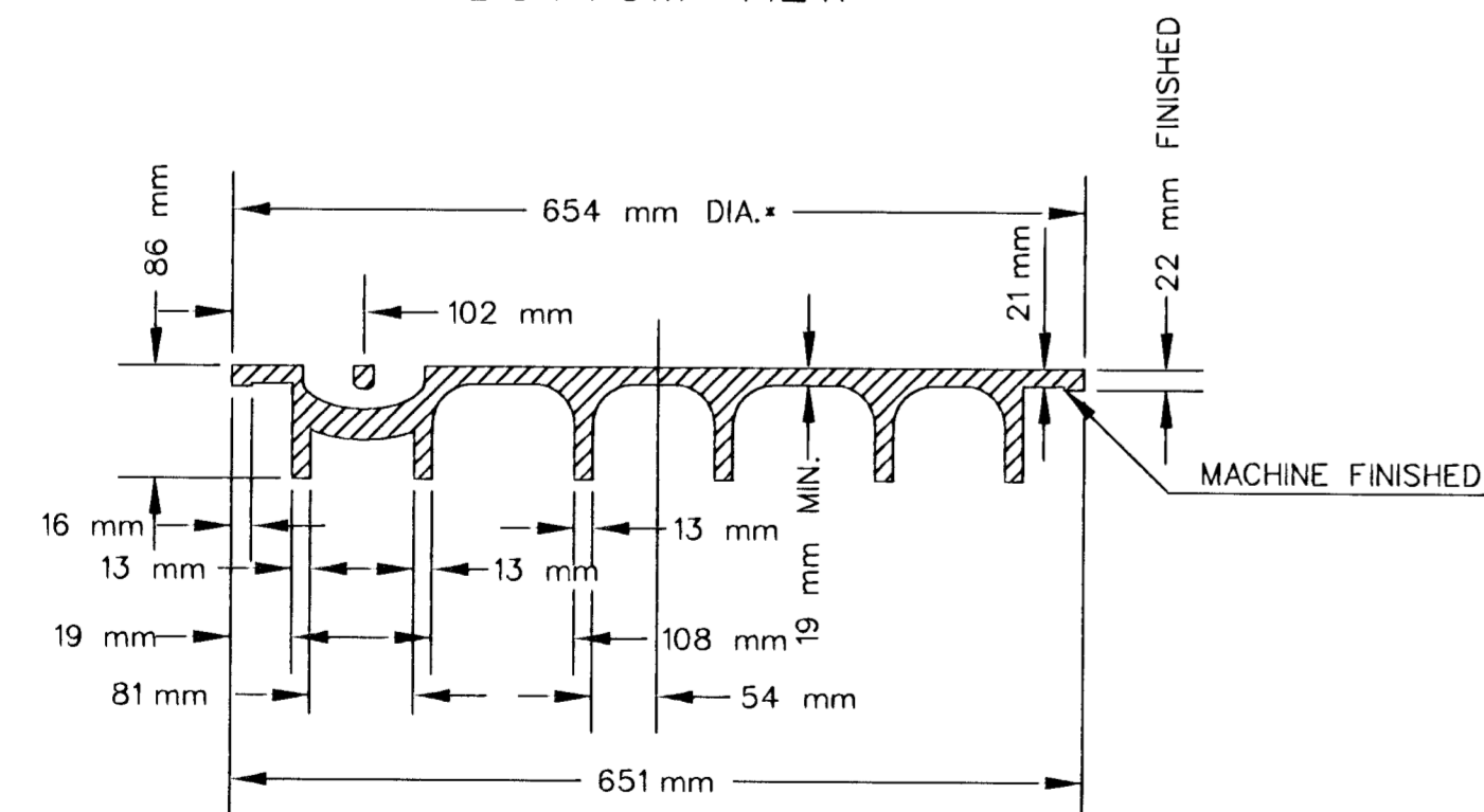
SECTION VIEW
