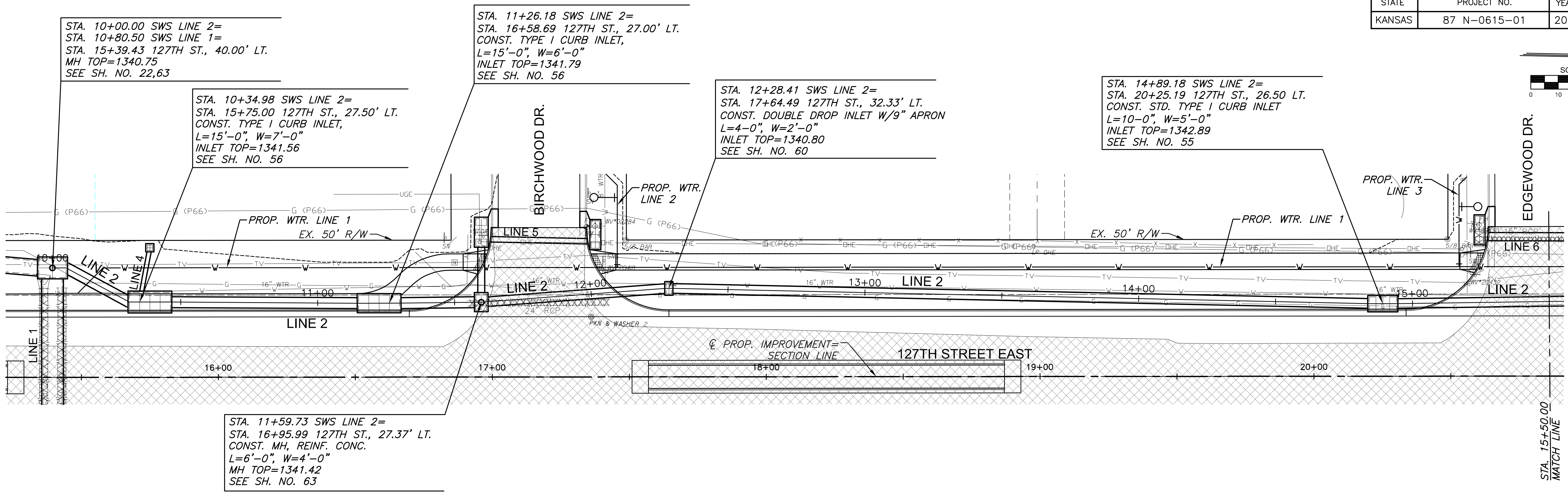
PLAN - LINE 2 PROFILE - LINE 2 SCALE: HORIZ. 1"=20' SCALE: VERT. 1"=5'
