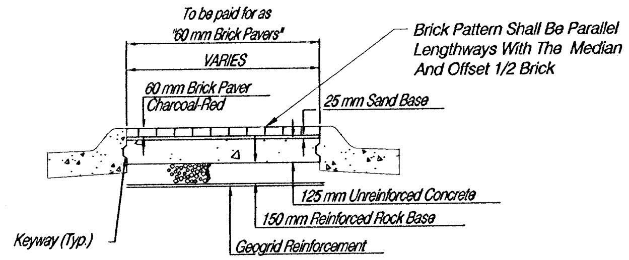
BRICK PAVER SURFACE DETAIL
