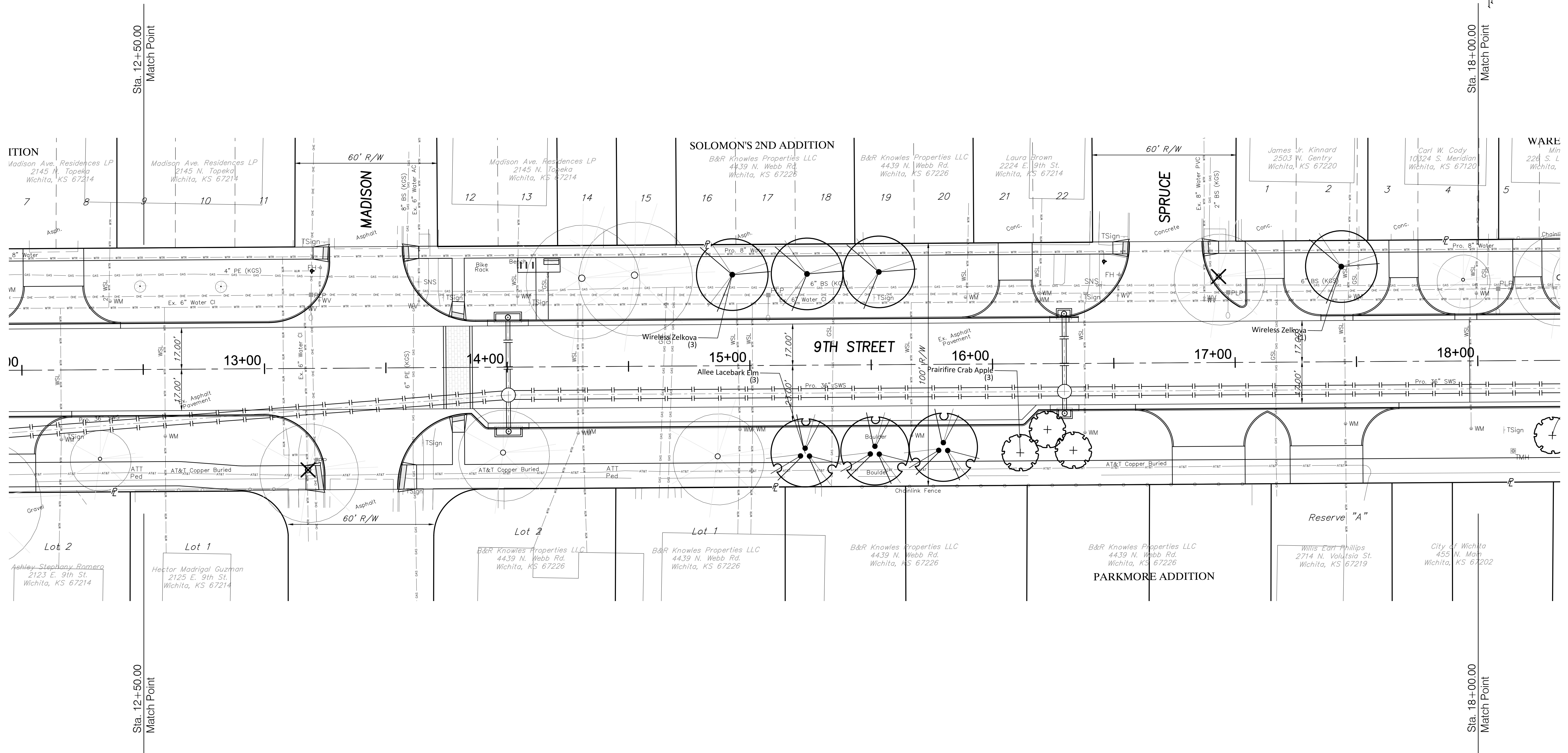
PLANT SCHEDULE 12+50 TO 18+00
