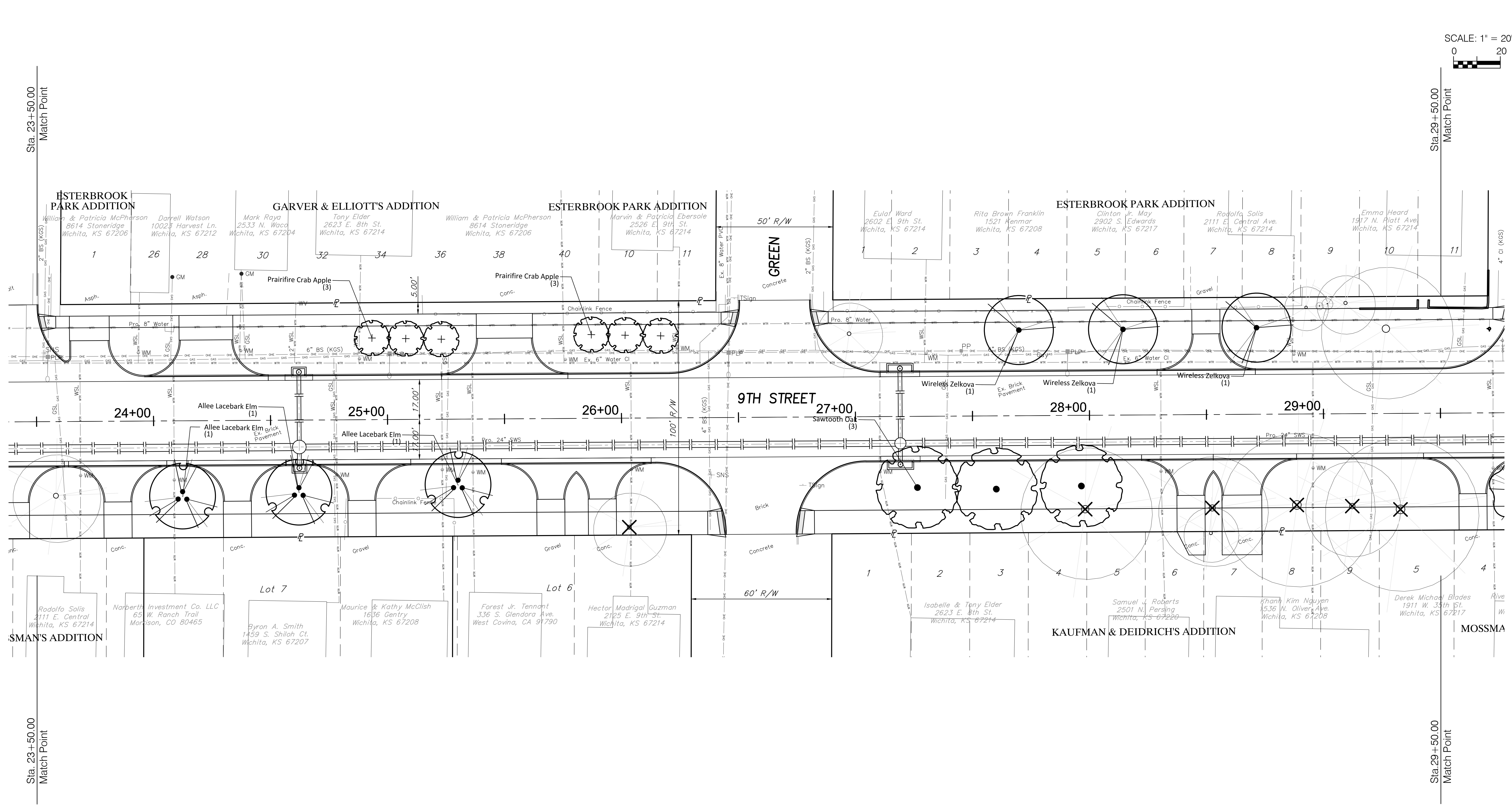
PLANT SCHEDULE 23+50 TO 29+50
