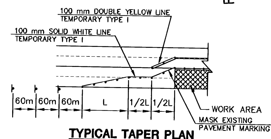
TYPICAL TAPER PLAN
