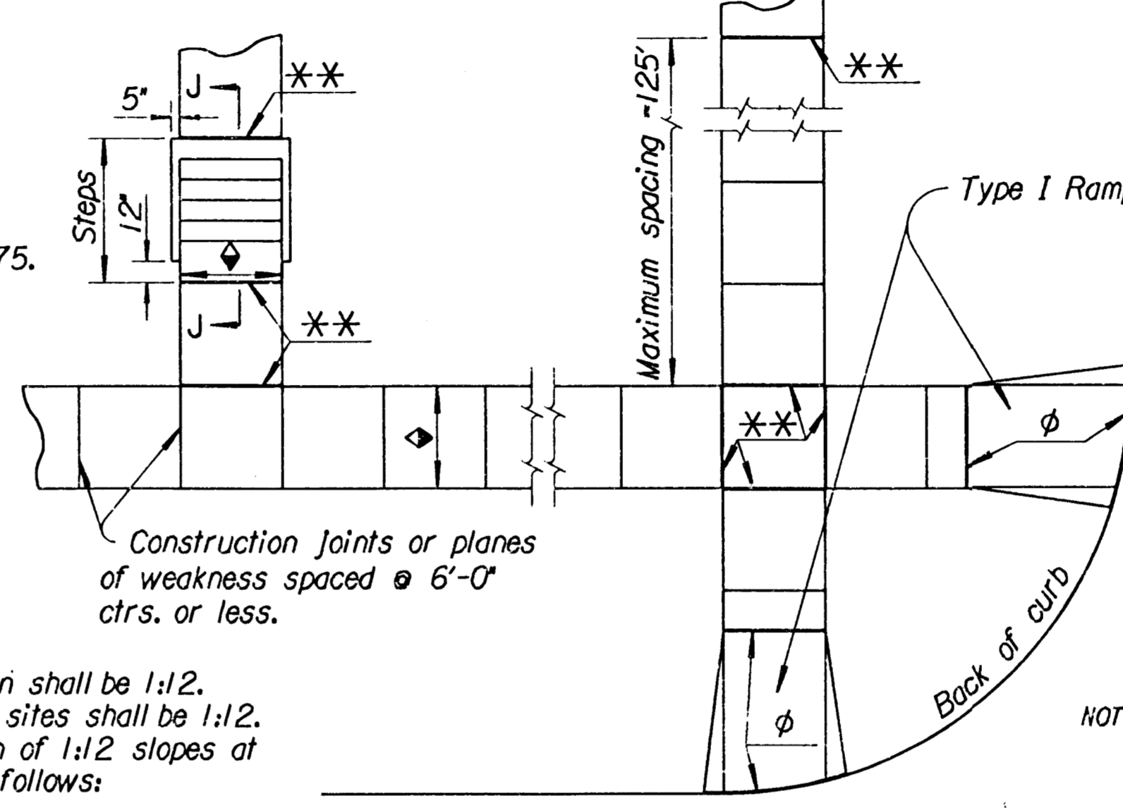
TYPICAL PLAN
