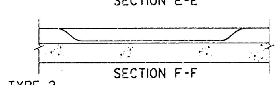
SECTION E-E
