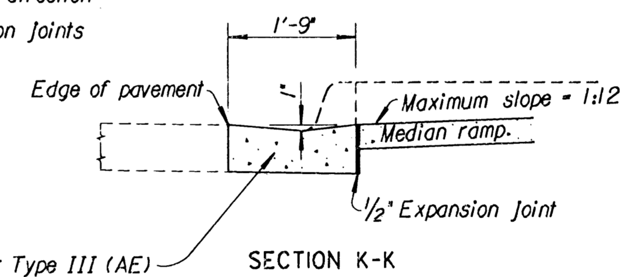
SECTION K-K
