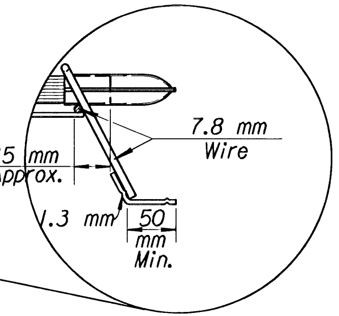
ALTERNATE WITH SAND PLATE
