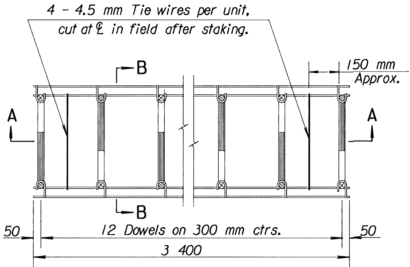
PLAN VIEW
