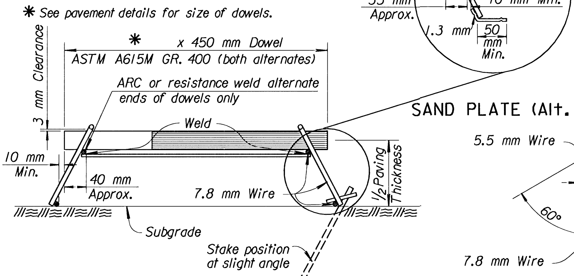
SEC. B-B
