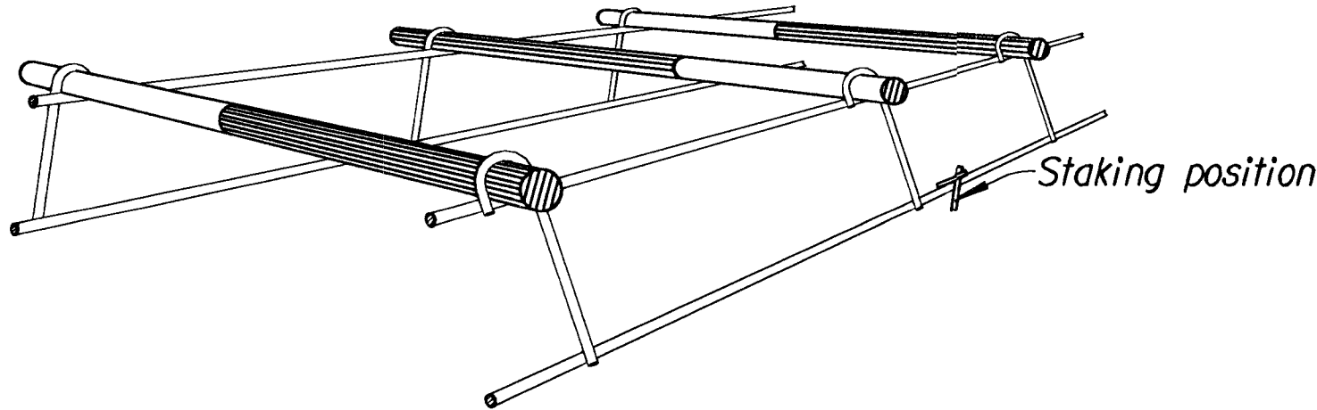
PERSPECTIVE VIEW
