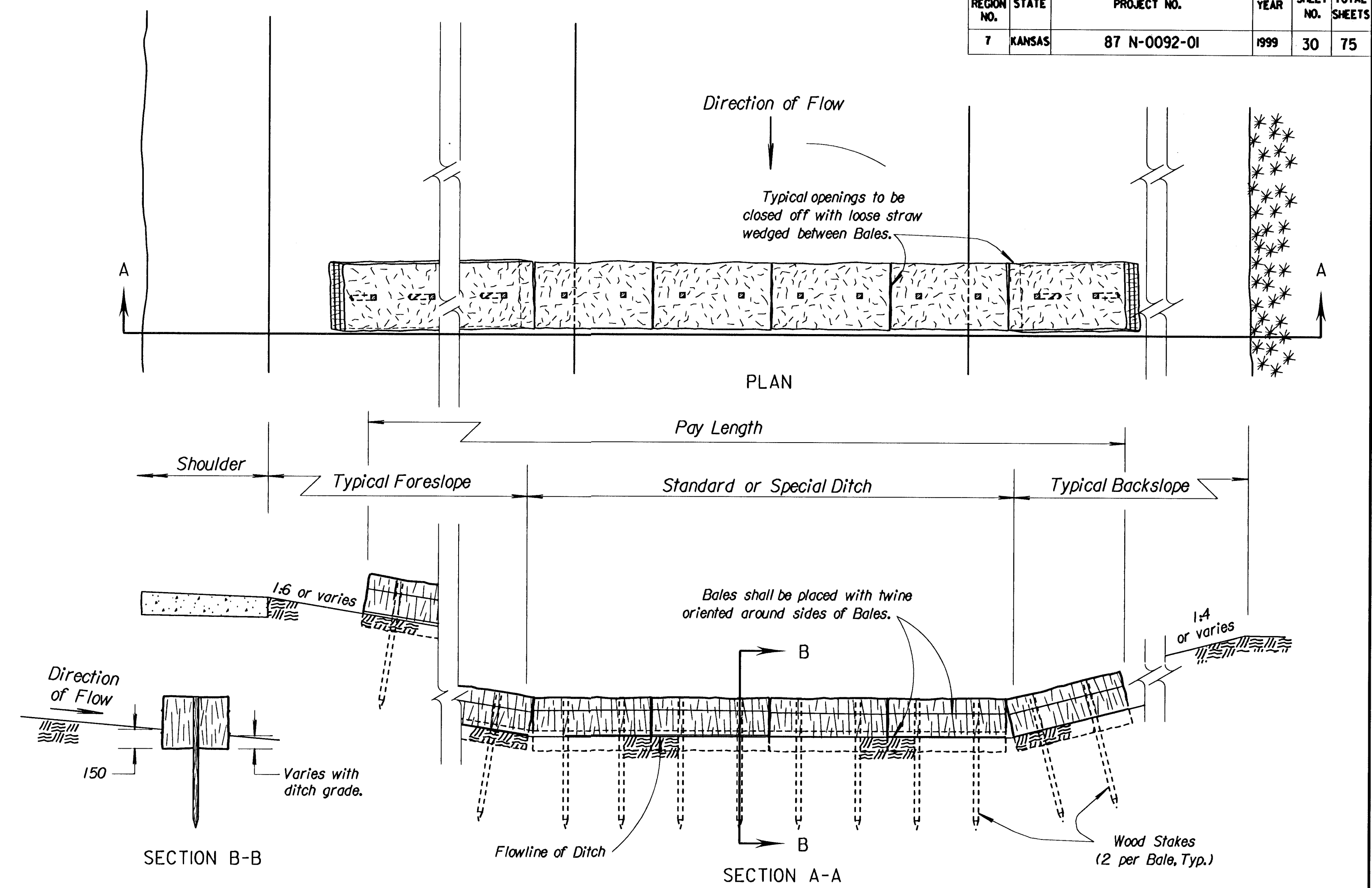
STRAW OR HAY BALE DITCH CHECK NO SCALE
