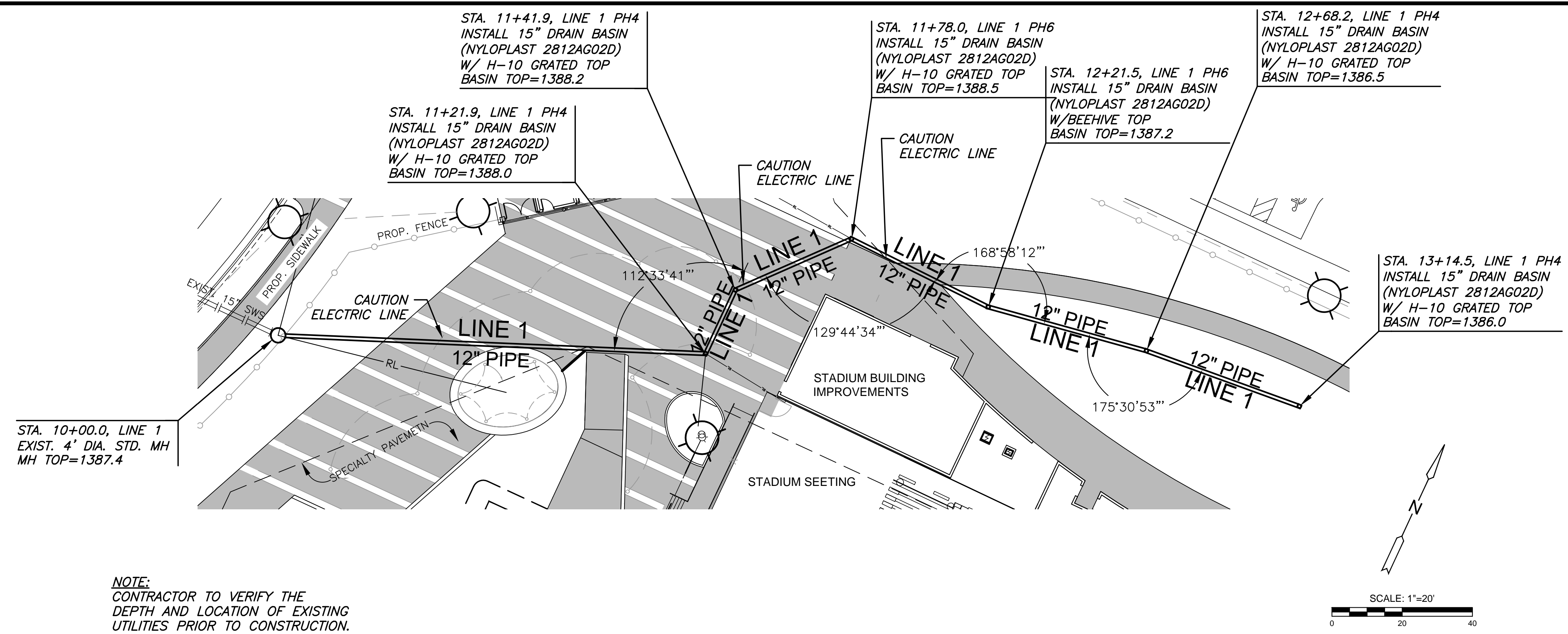
PLAN SWS LINE 1 PH6 PROFILE SWS LINE 1 PH6
