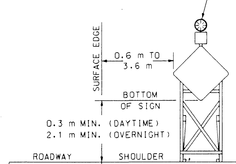
HEIGHT AND LATERAL DIMENSIONS FOR SIGNS MOUNTED ON SKIDS OR OTHER MOVABLE MOUNTS
