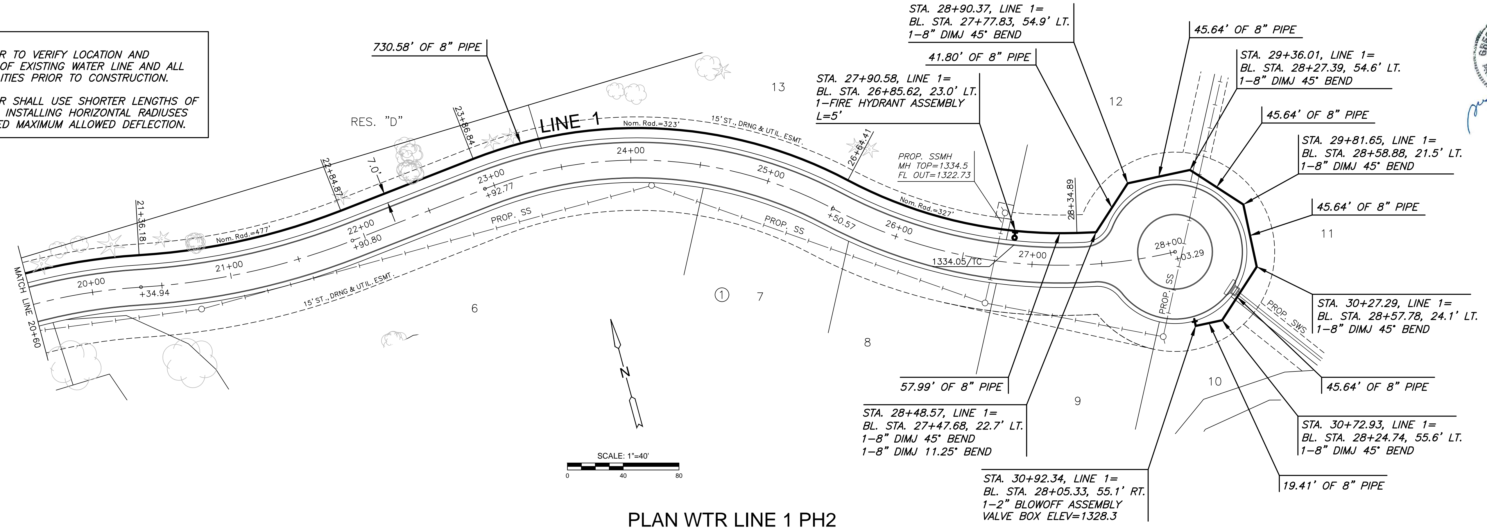
PLAN WTR LINE 1 PH2 PROFILE WTR LINE 1 PH2
