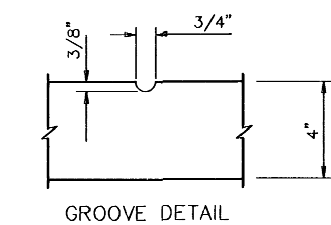
GROOVE DETAIL
