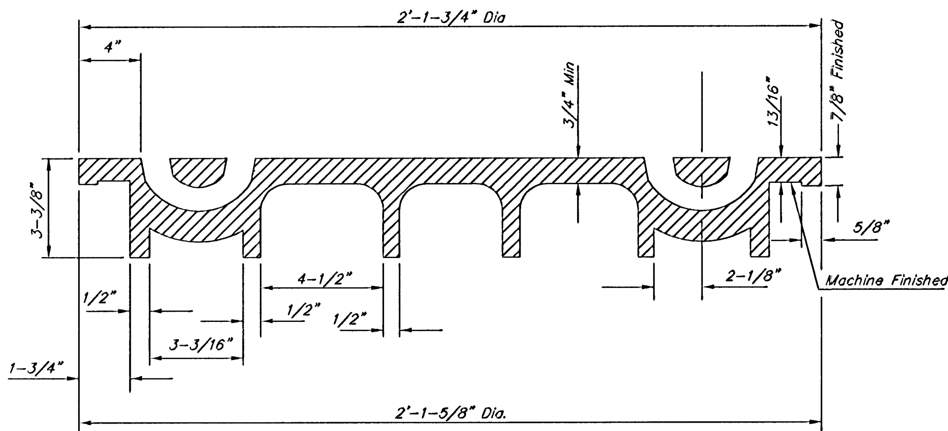
SECTION VIEW
