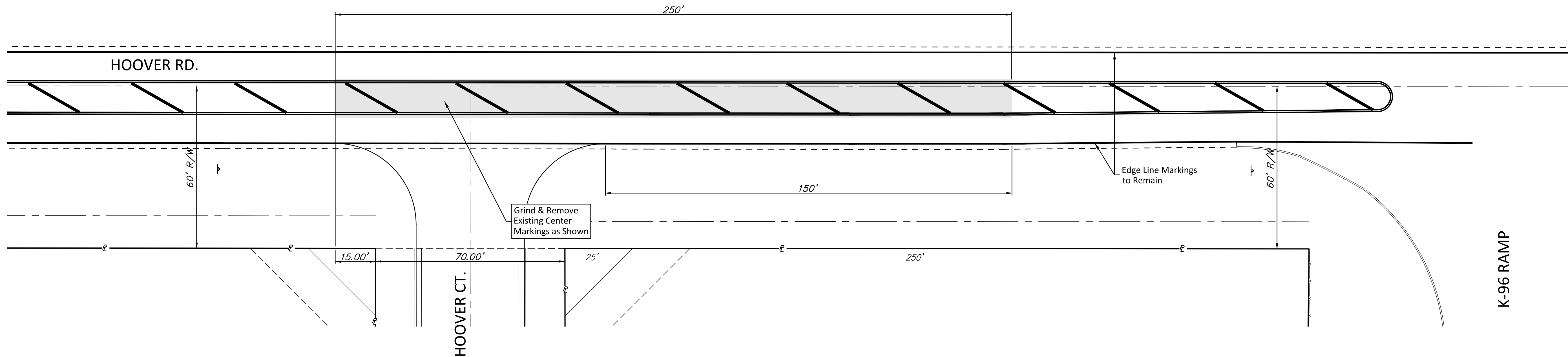
EXISTING MARKINGS - DEMO 1"=20'
