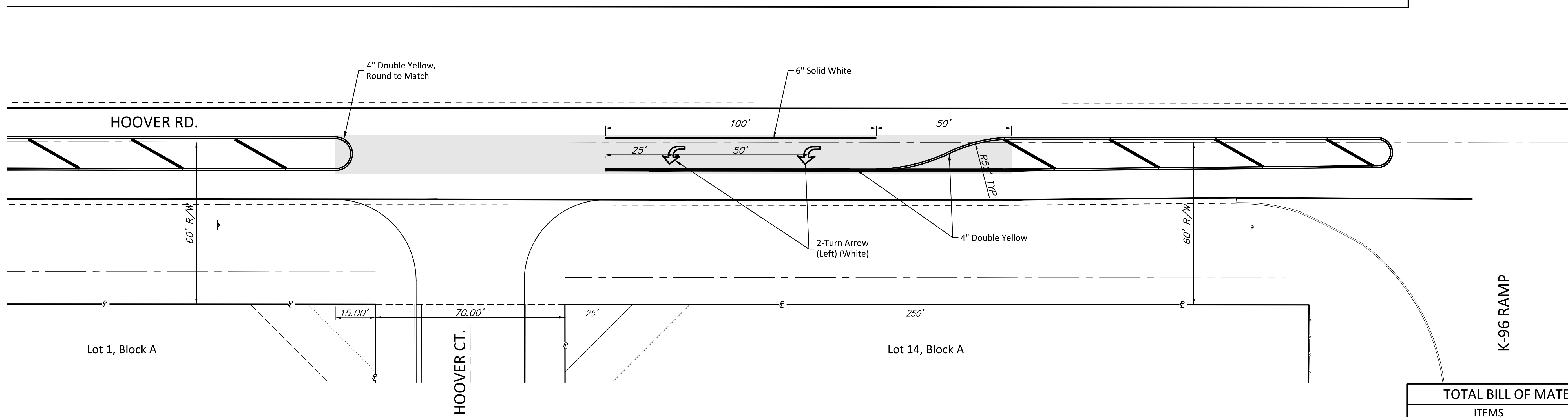
PROPOSED MARKINGS 1"=20'
