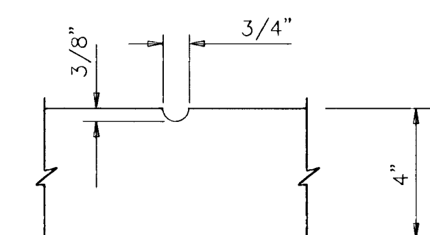
GROOVE DETAIL
