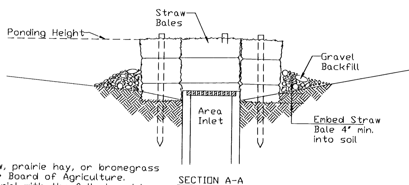
STRAW BALE BARRIERS FOR AREA INLETS (INLET PROTECTION)
