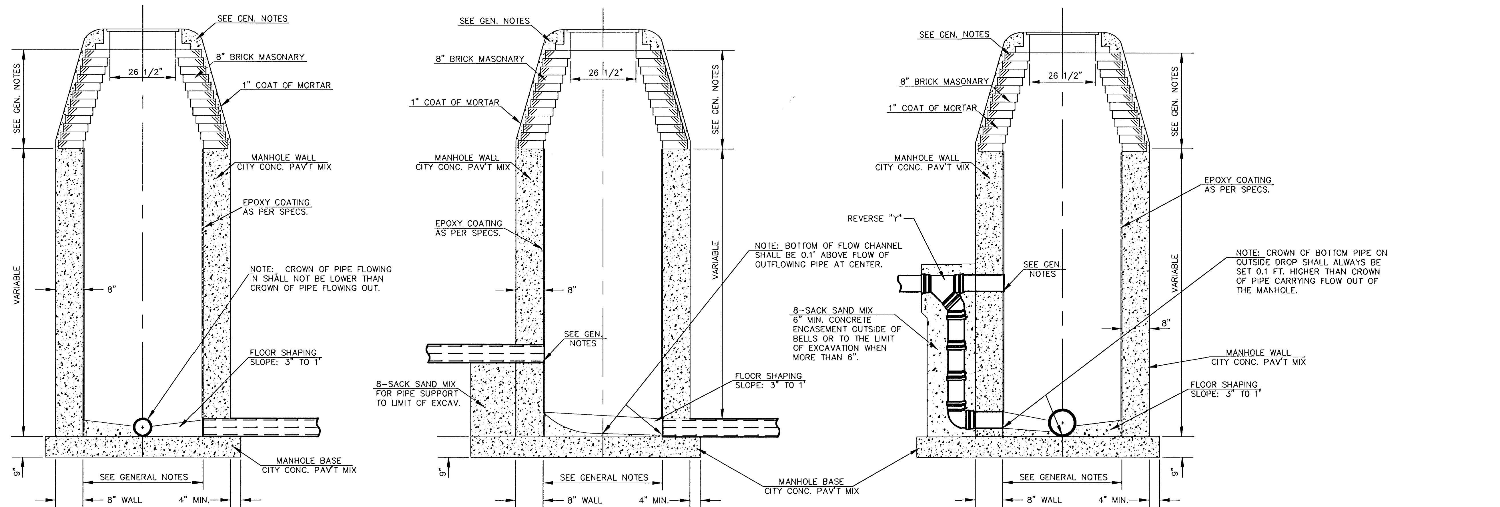
OUTSIDE DROP MANHOLE TYPE "D"
