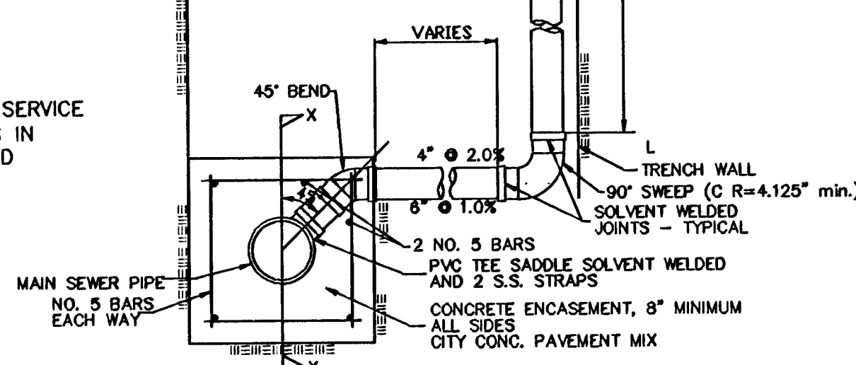
TYPICAL RISER DETAIL
