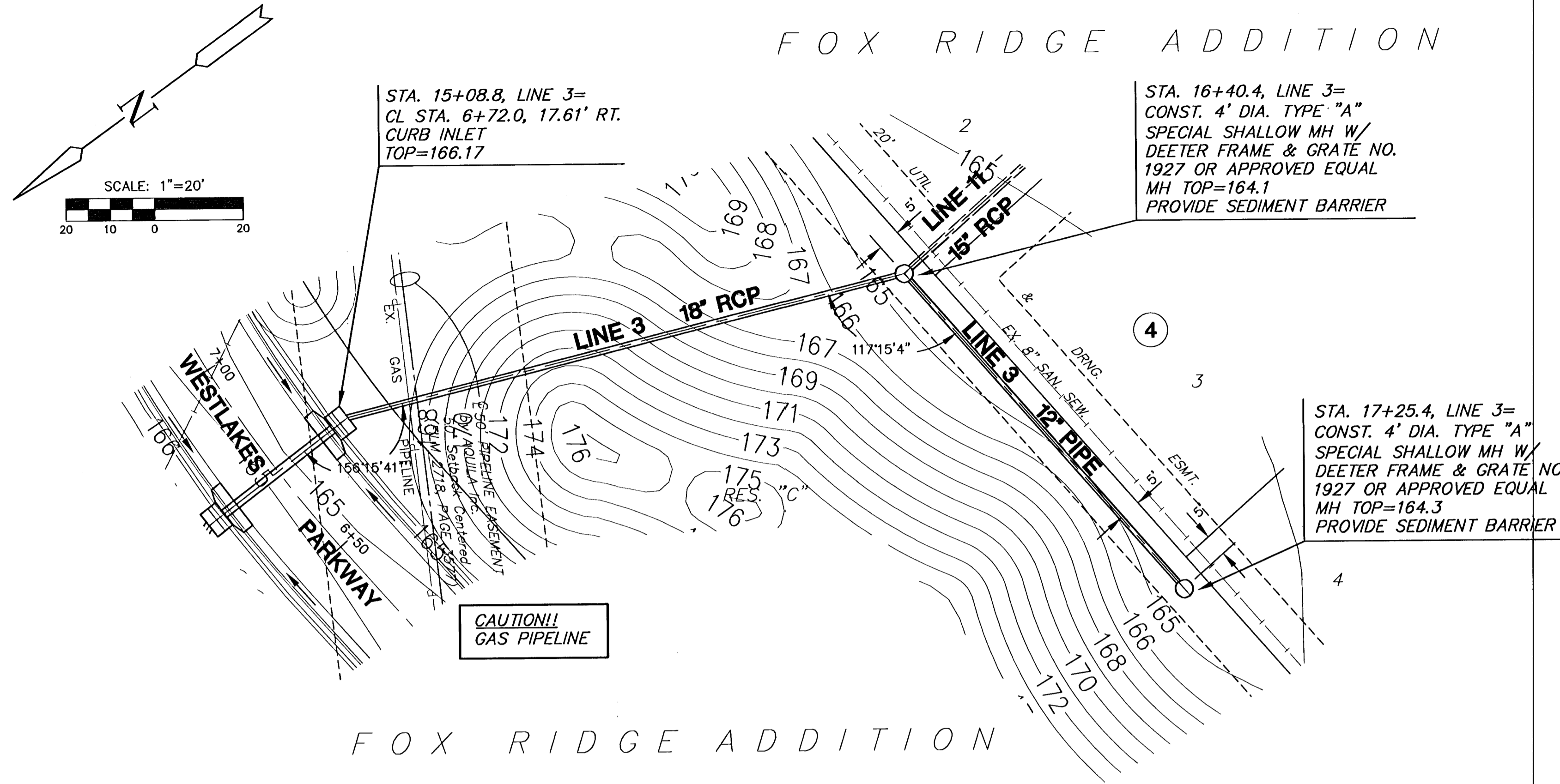
PLAN LINE 3
