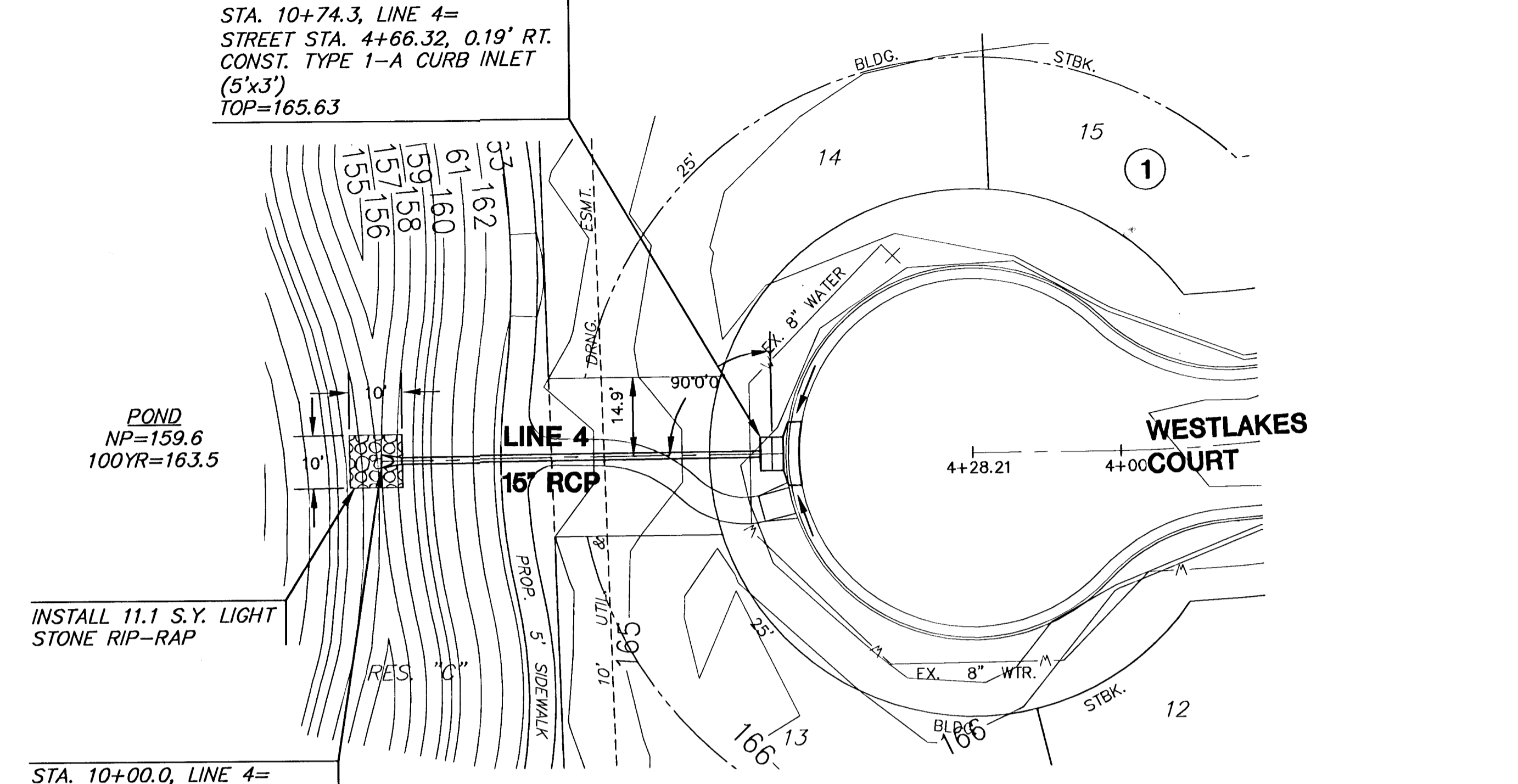
PLAN LINE 4
