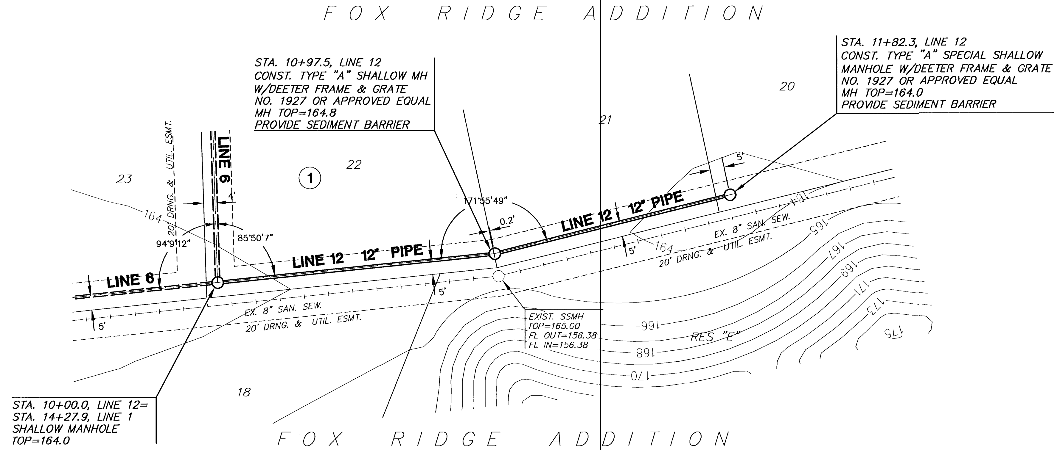
PLAN LINE 12
