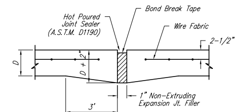
EXPANSION JOINT
