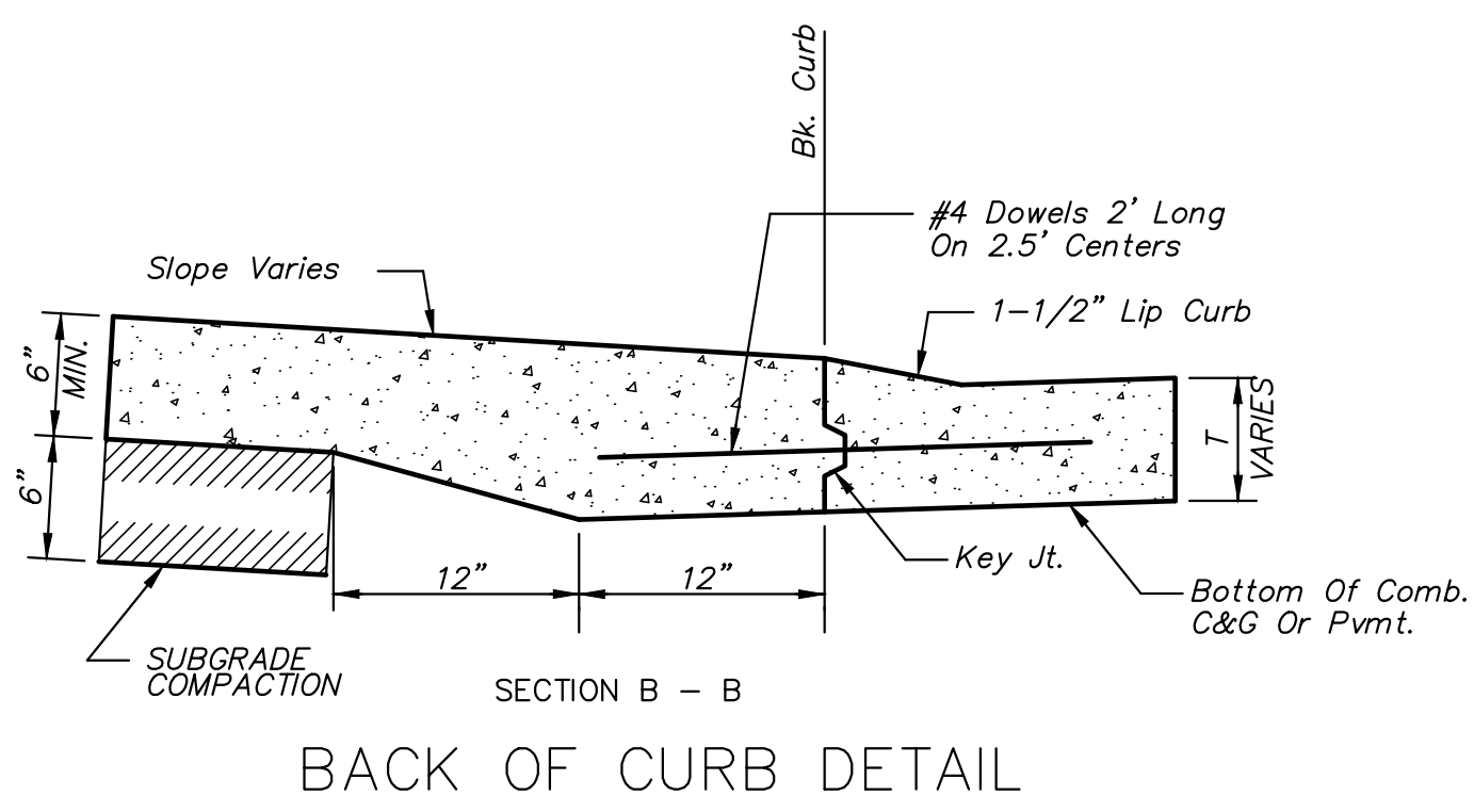
Combined Curb & Gutter (1 1/2")
