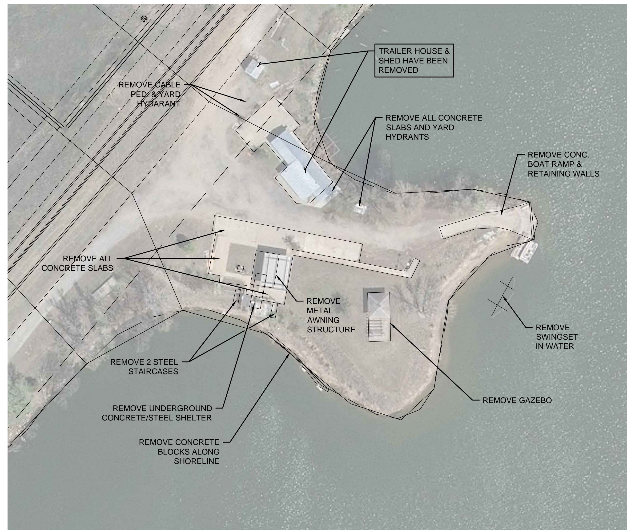
DEMO PLAN - LOT 9, BLOCK 1 (SUBSIDIARY TO SITE CLEARING)
