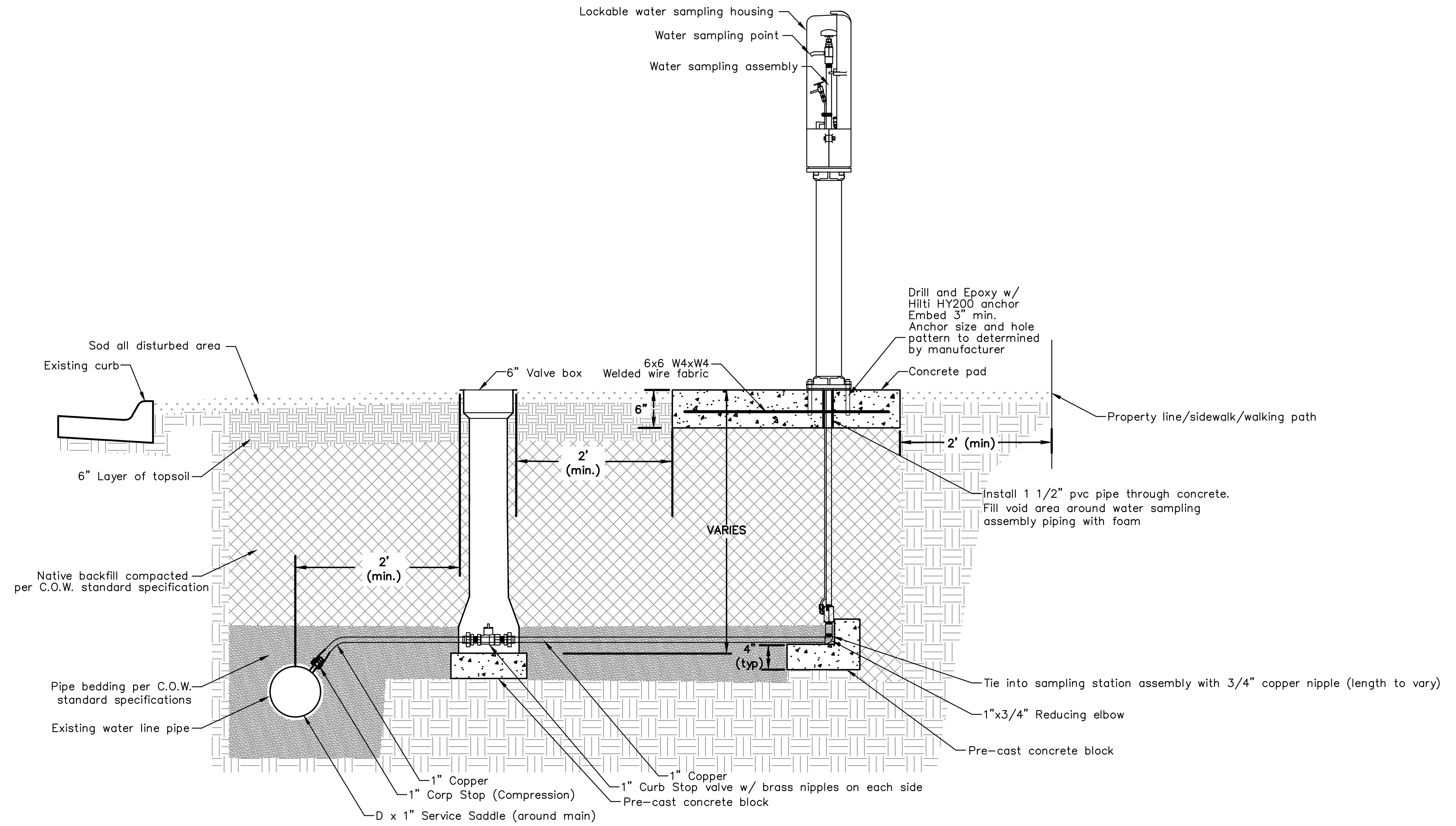
Profile View - Section A-A
