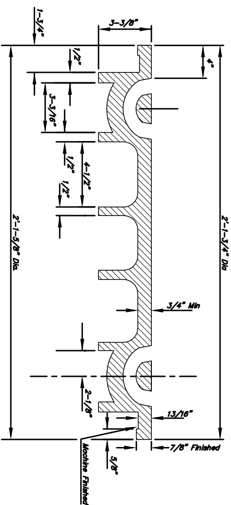
SECTION VIEW
