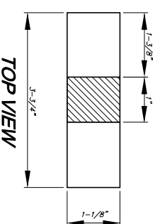
PICKHOLE DETAIL
