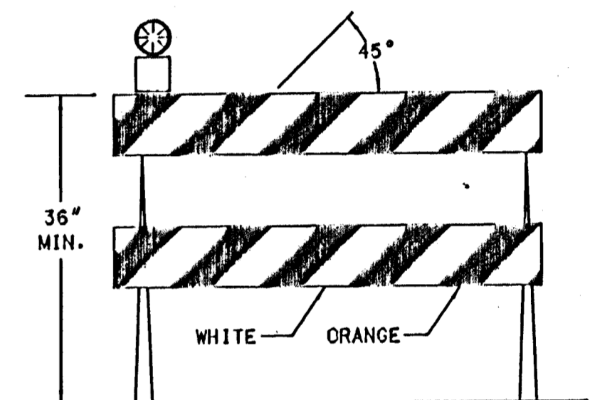
TYPE II BARRICADE WITH LIGHT
