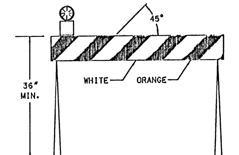
TYPE I BARRICADE WITH LIGHT
