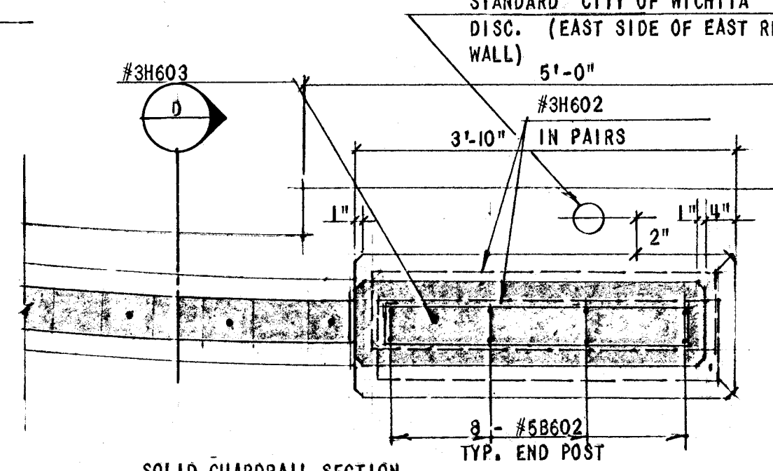
SOLID GUARDRAIL SECTION - TYP. OF 2 SECTIONS AT END OF GUARDRAIL
