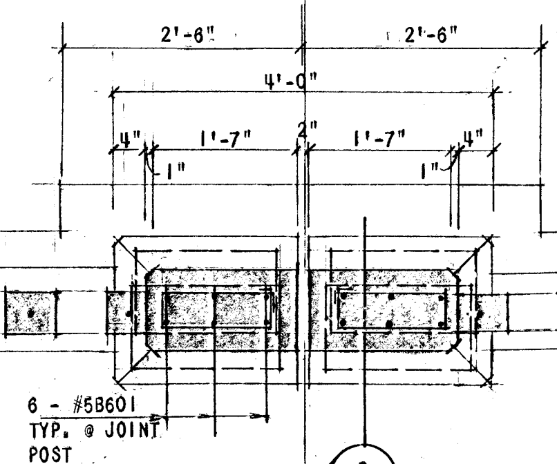
TYPICAL JOINT POST
