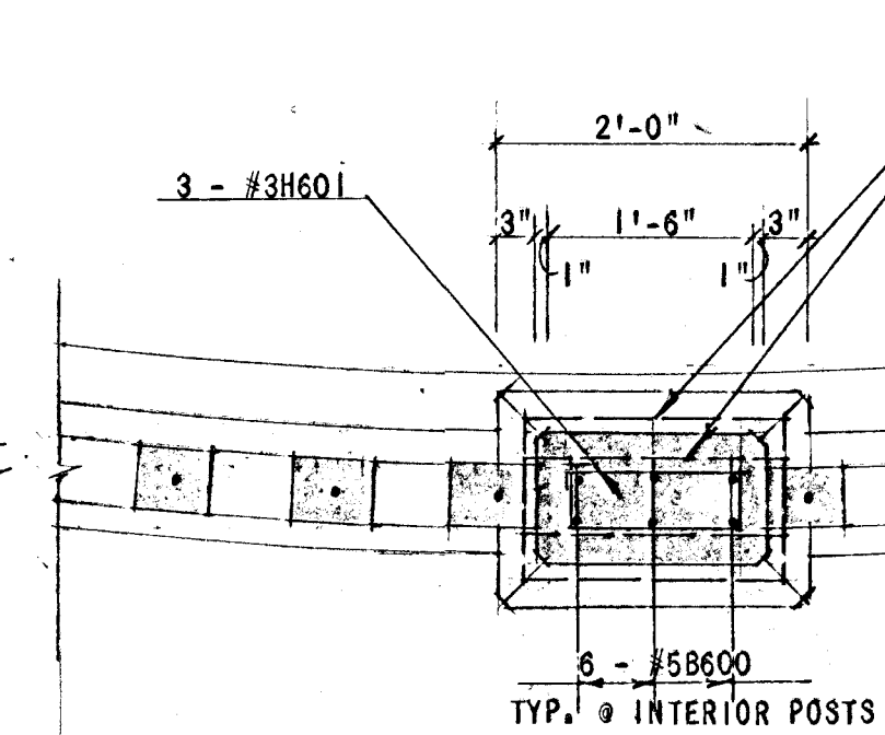
TYPICAL INTERIOR POST ON BRIDGE AND WALL AREA
