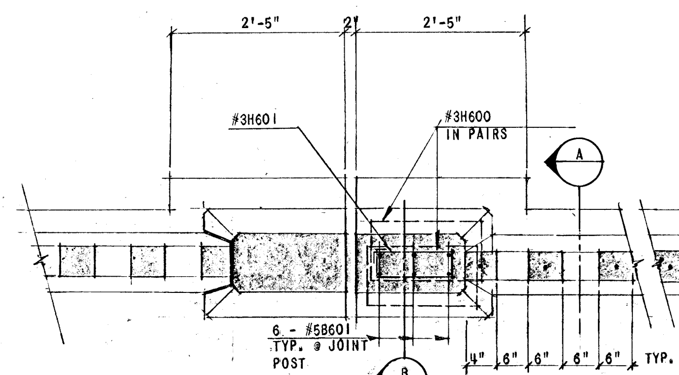
GUARDRAIL PLAN SECTION
