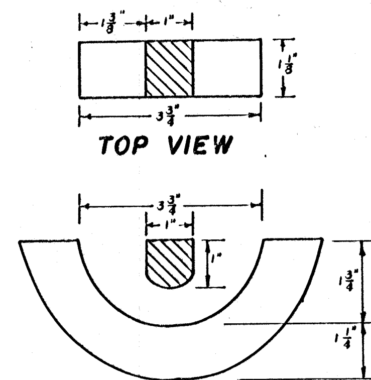
SECTION VIEW
