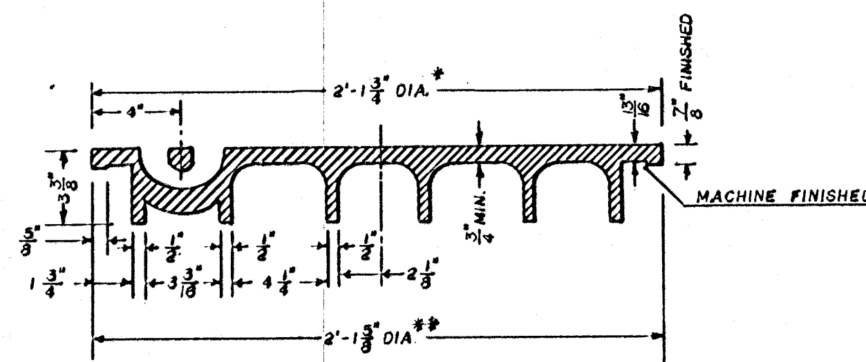
SECTION VIEW
