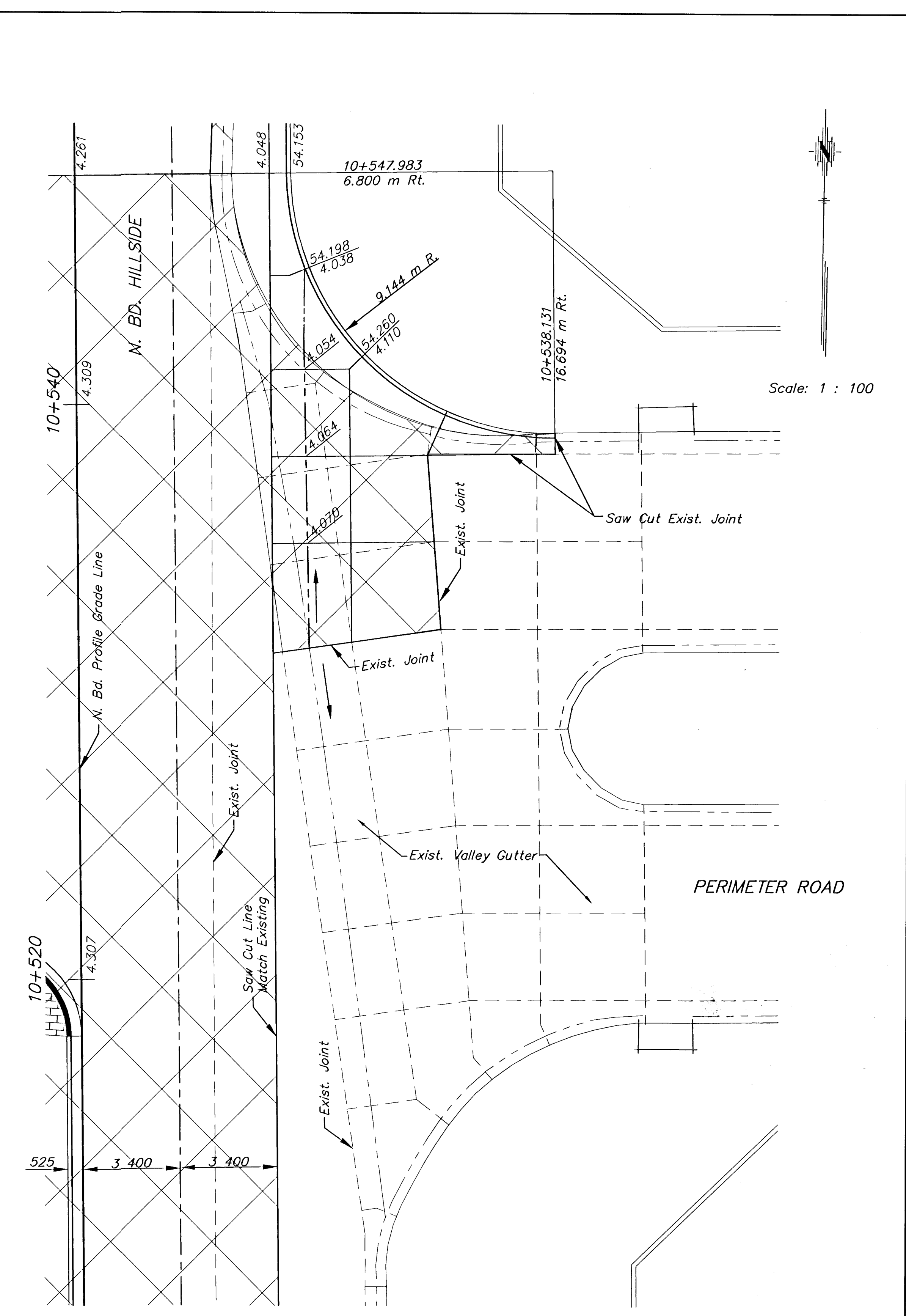
PLAN - HILLSIDE & PERIMETER ROAD
