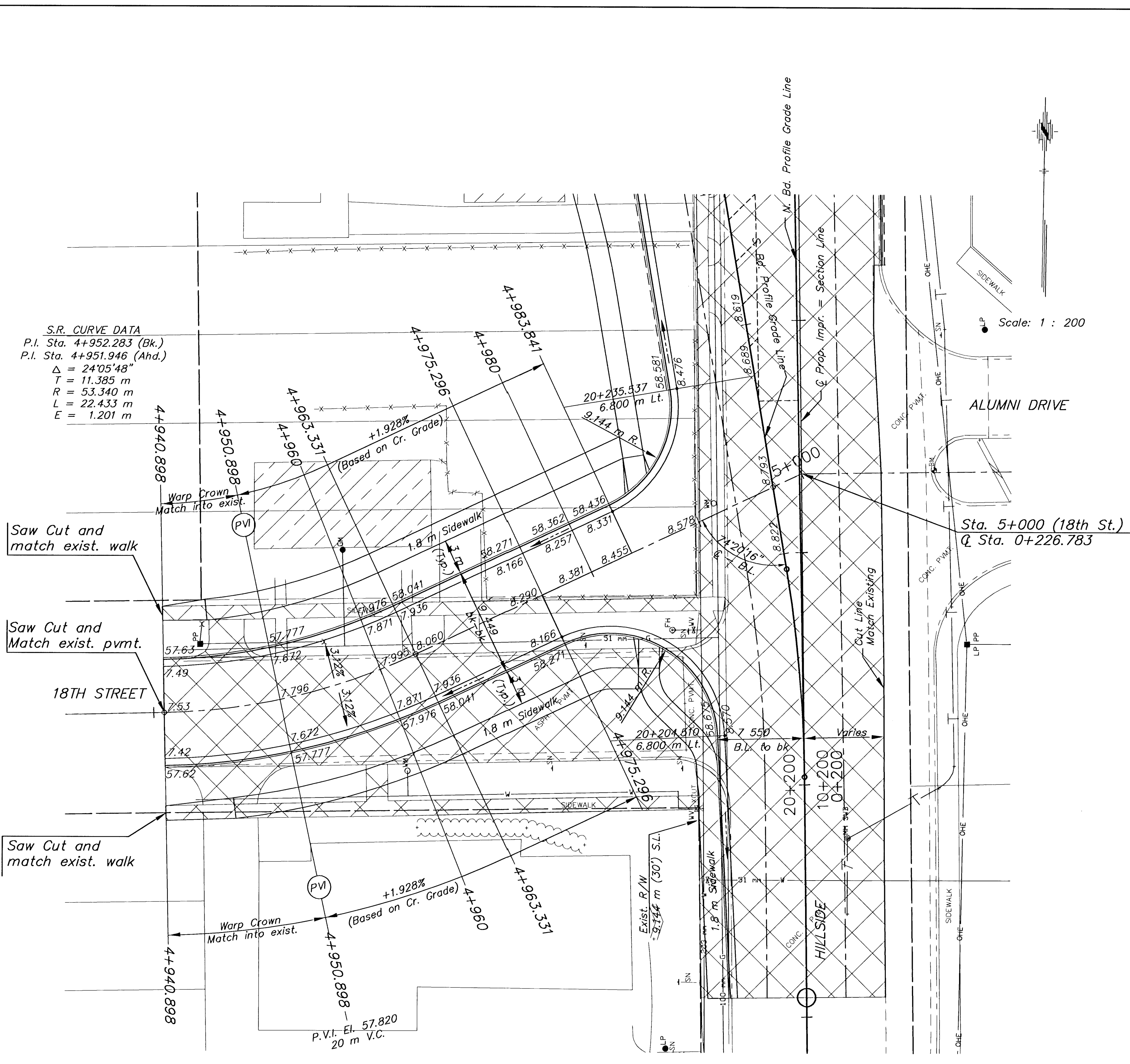
PLAN - HILLSIDE & 18TH STREET
