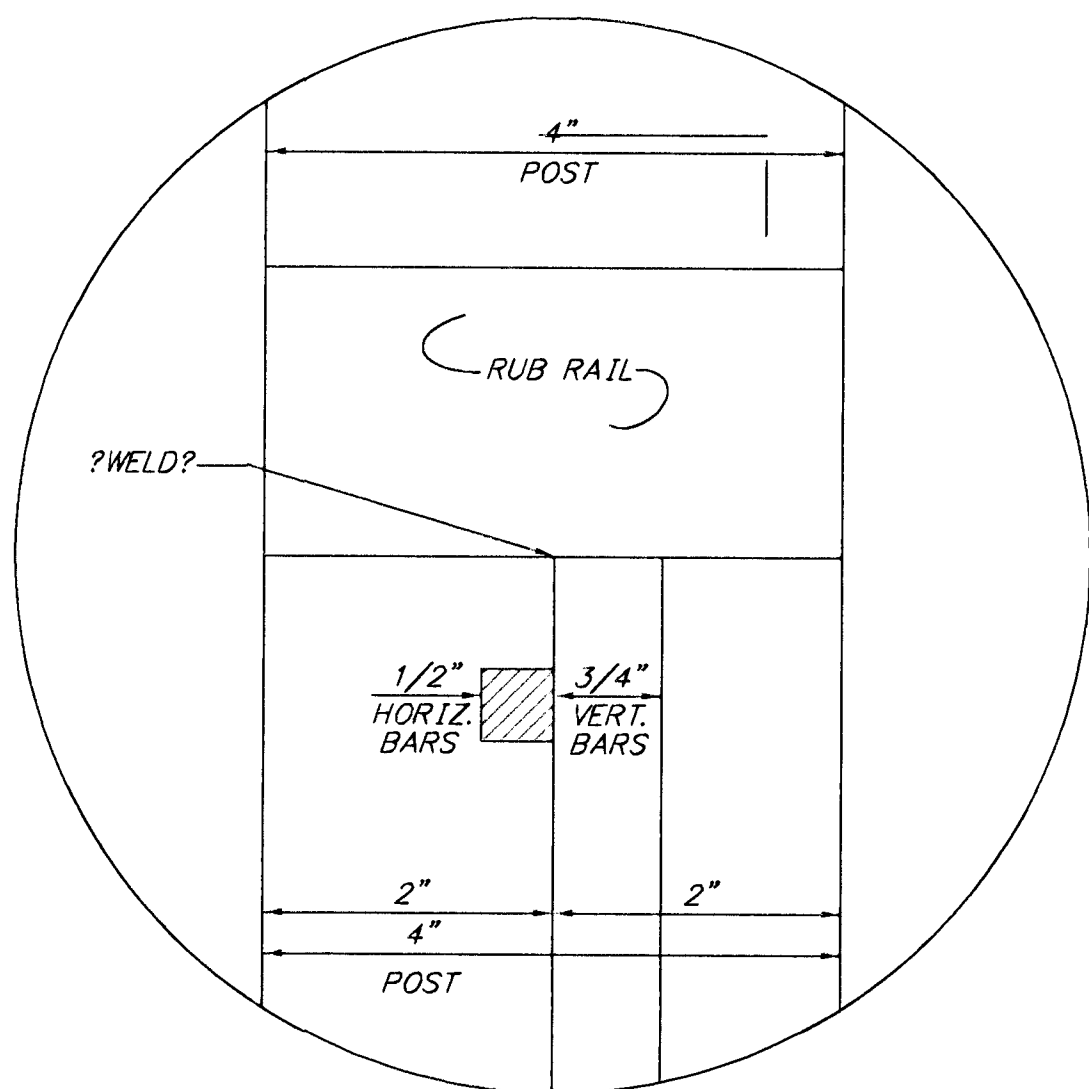
PICKET DETAIL NO SCALE
