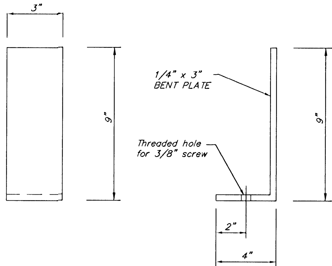
HANDRAIL BASE PLATE NO SCALE
