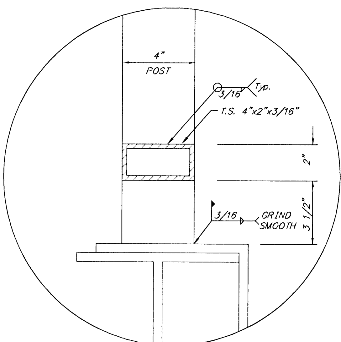
BOTTOM HANDRAIL DETAIL NO SCALE
