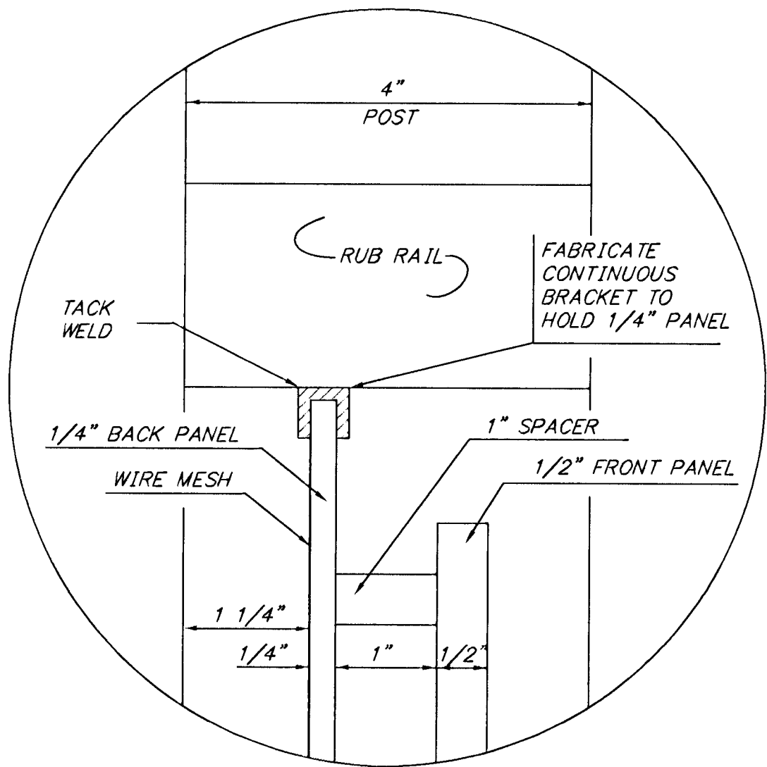
PANEL INSERT DETAIL NO SCALE
