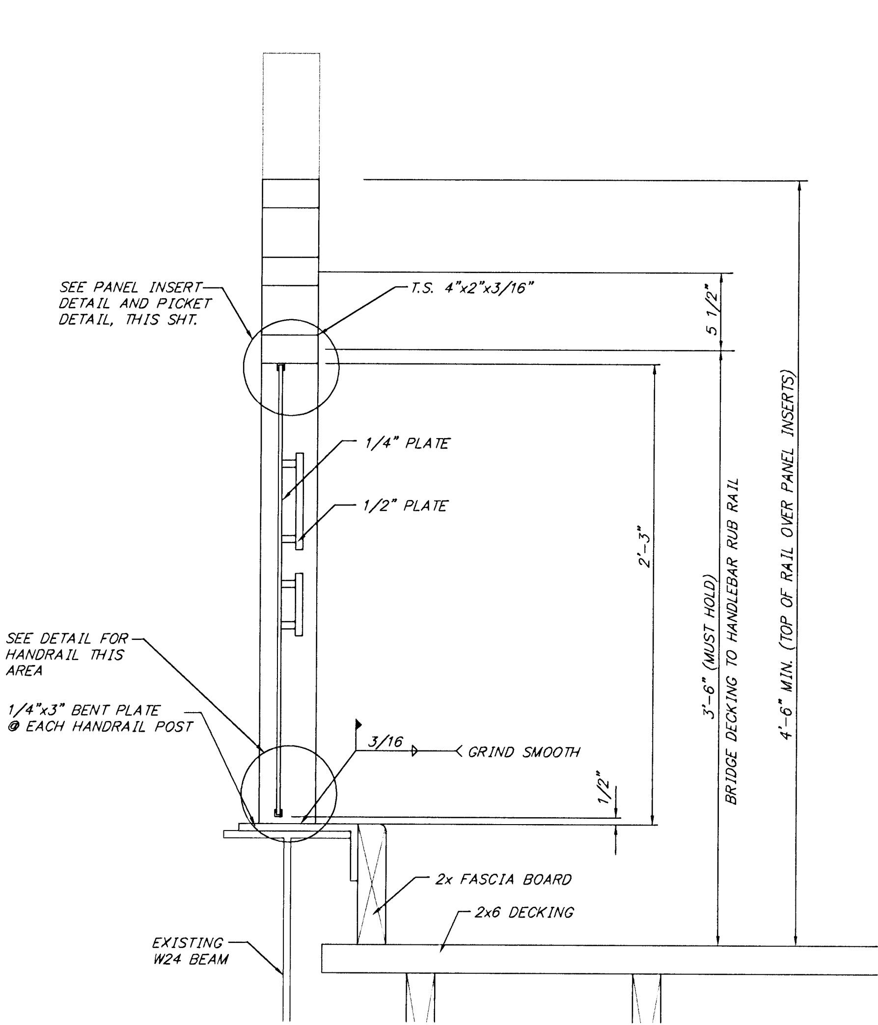
HANDRAIL SECTION NO SCALE
