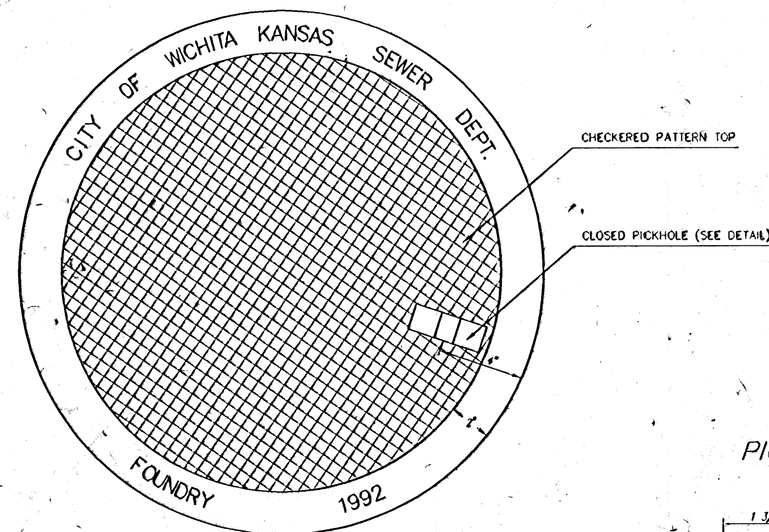
TOP VIEW
