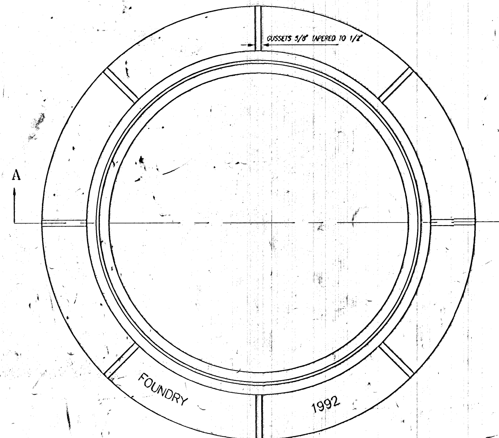
TOP VIEW
