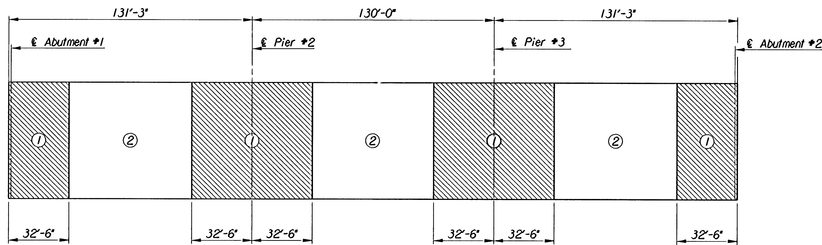
CONCRETE PLACING SEQUENCE
