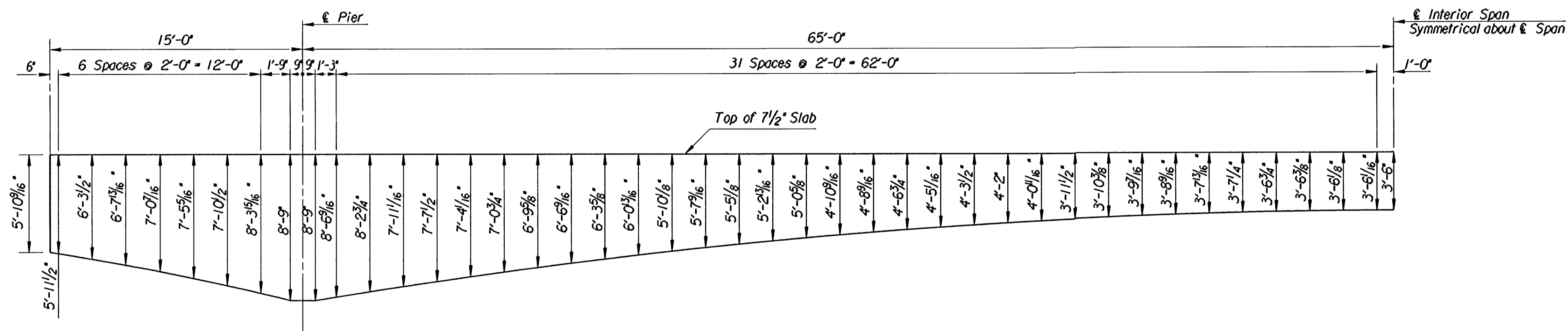
BEAM ORDINATES Along \epsilon Beam
