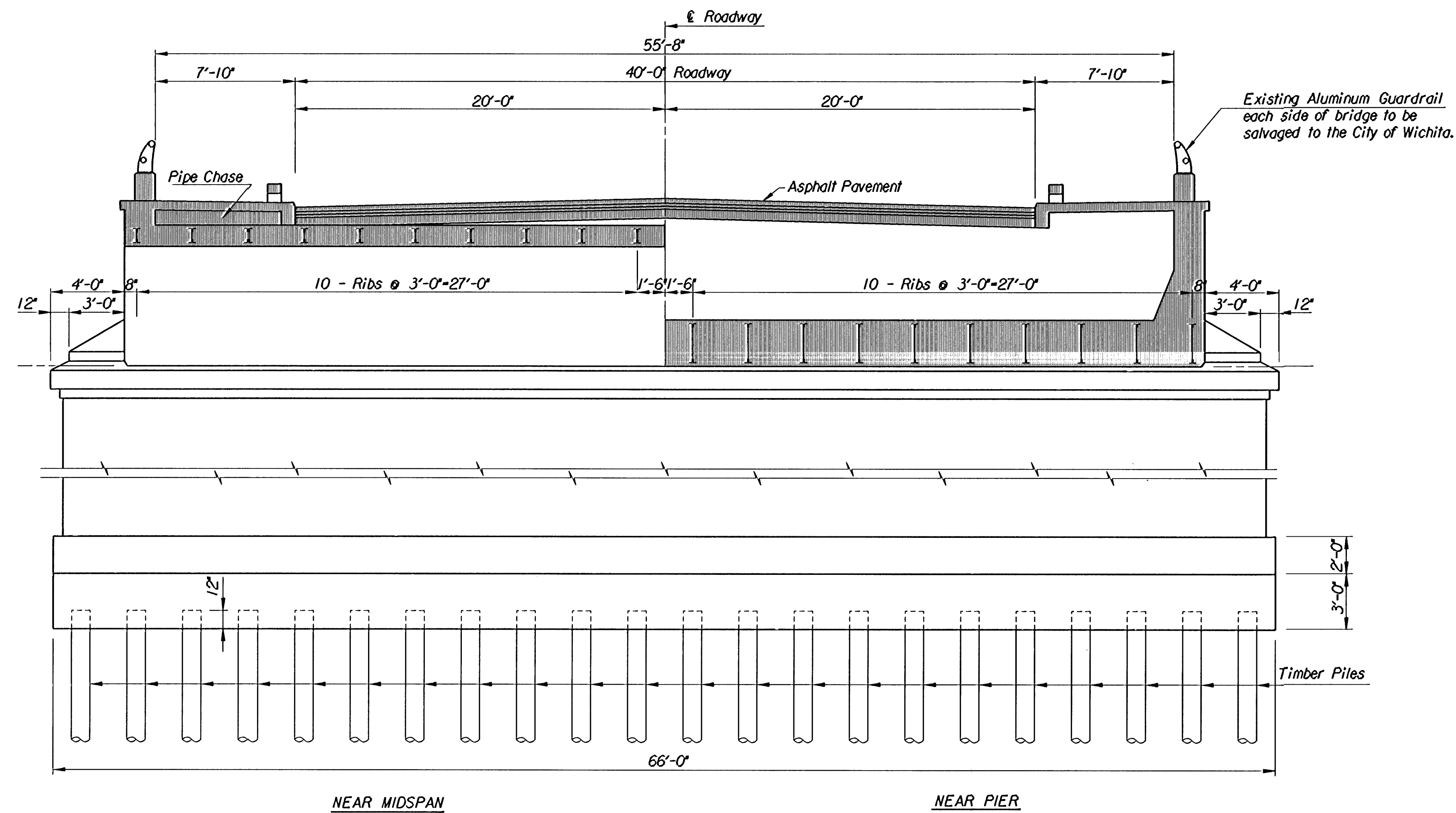
TYPICAL ELEVATION Note: Existing pipe poles and cables for seasonal lighting to be salvaged to the City of Wichita.
