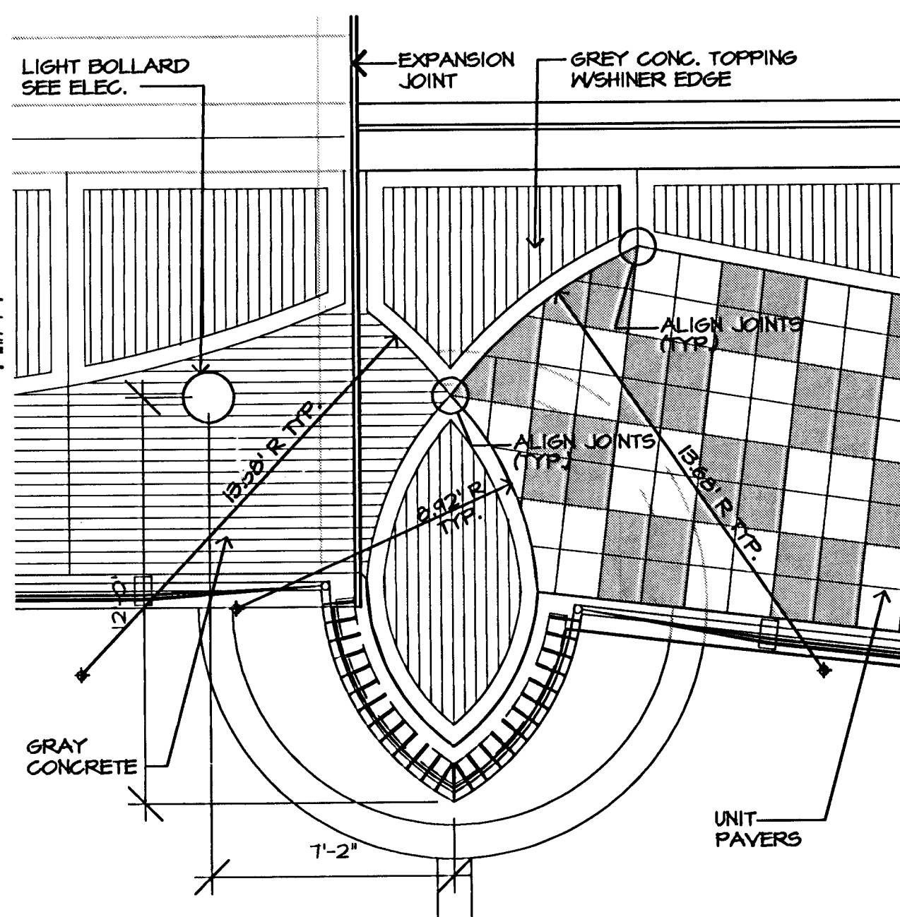
C ENLARGED CONC. PAVING & PIER LOOKOUTS TYP. 4 LOCATIONS 0' 2' 4' 6' 1/4"=1'-0"
