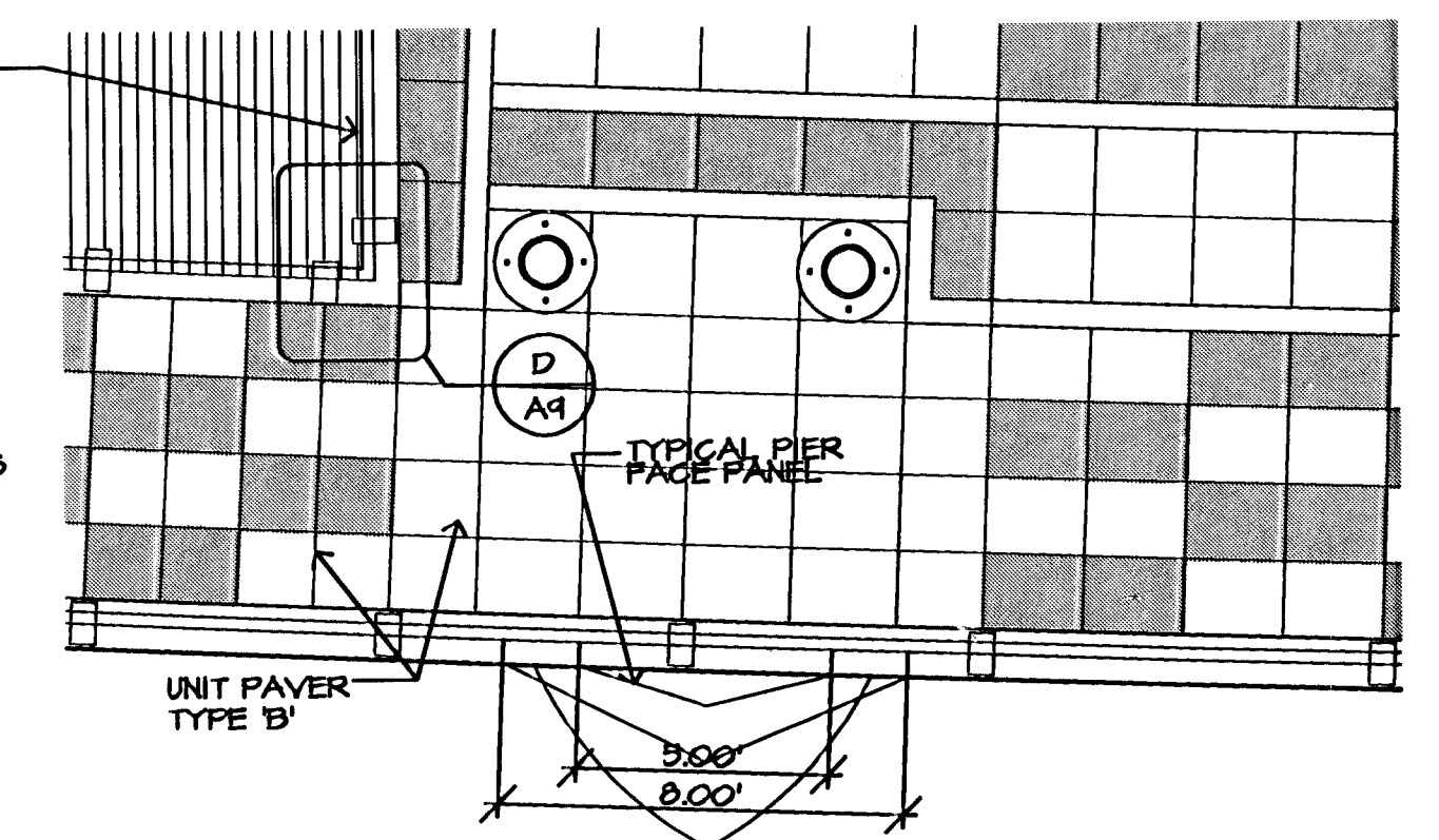
E ENLARGED PIER LOOKOUT PLAN TYP. 4 PLACES, SOUTHWEST LOCATION INDICATED 0' 2' 4' 6' 1/4"=1'-0"
