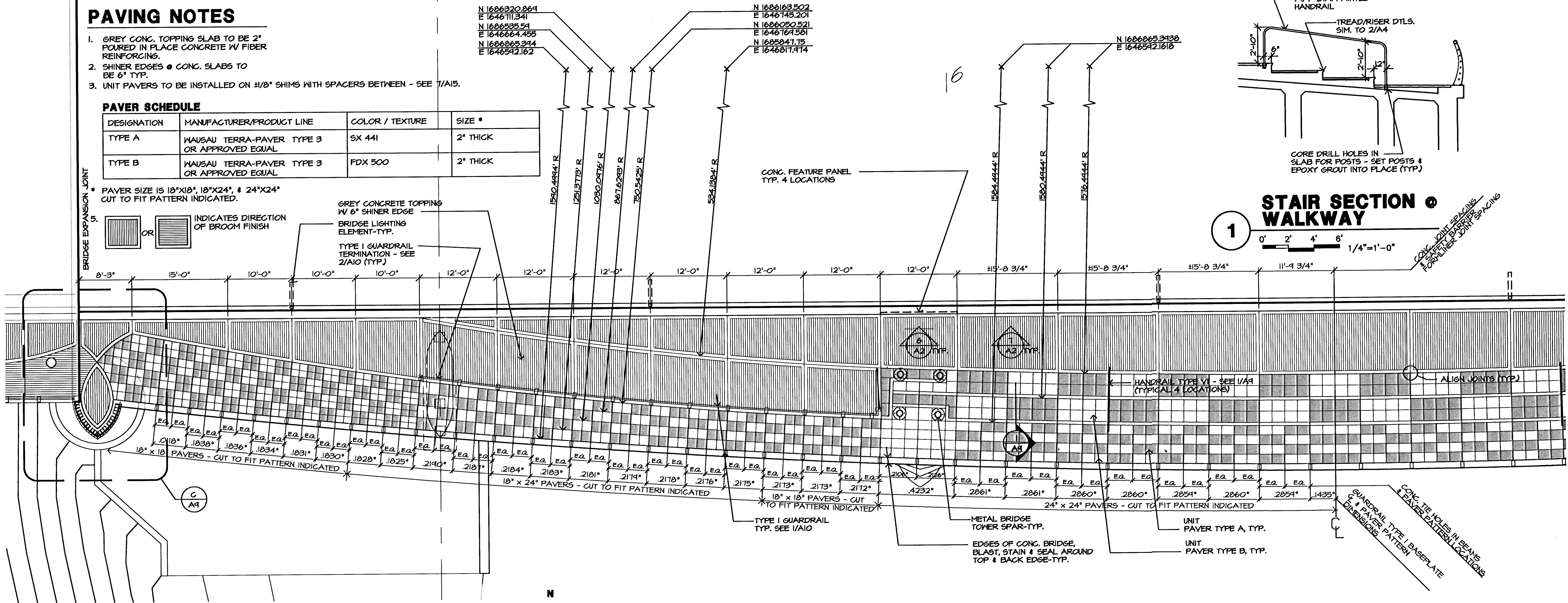
A ENLARGED PLAN TYPICAL HALF SPAN 0' 4' 8' 12' 1/8"=1'-0"
