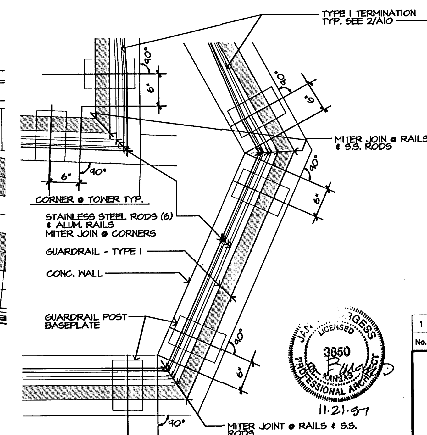
D ENLARGED CORNER PLAN GUARDRAIL TYPE I NORTHEAST LOCATION 0' 6' 1' 1"=1'-0"
