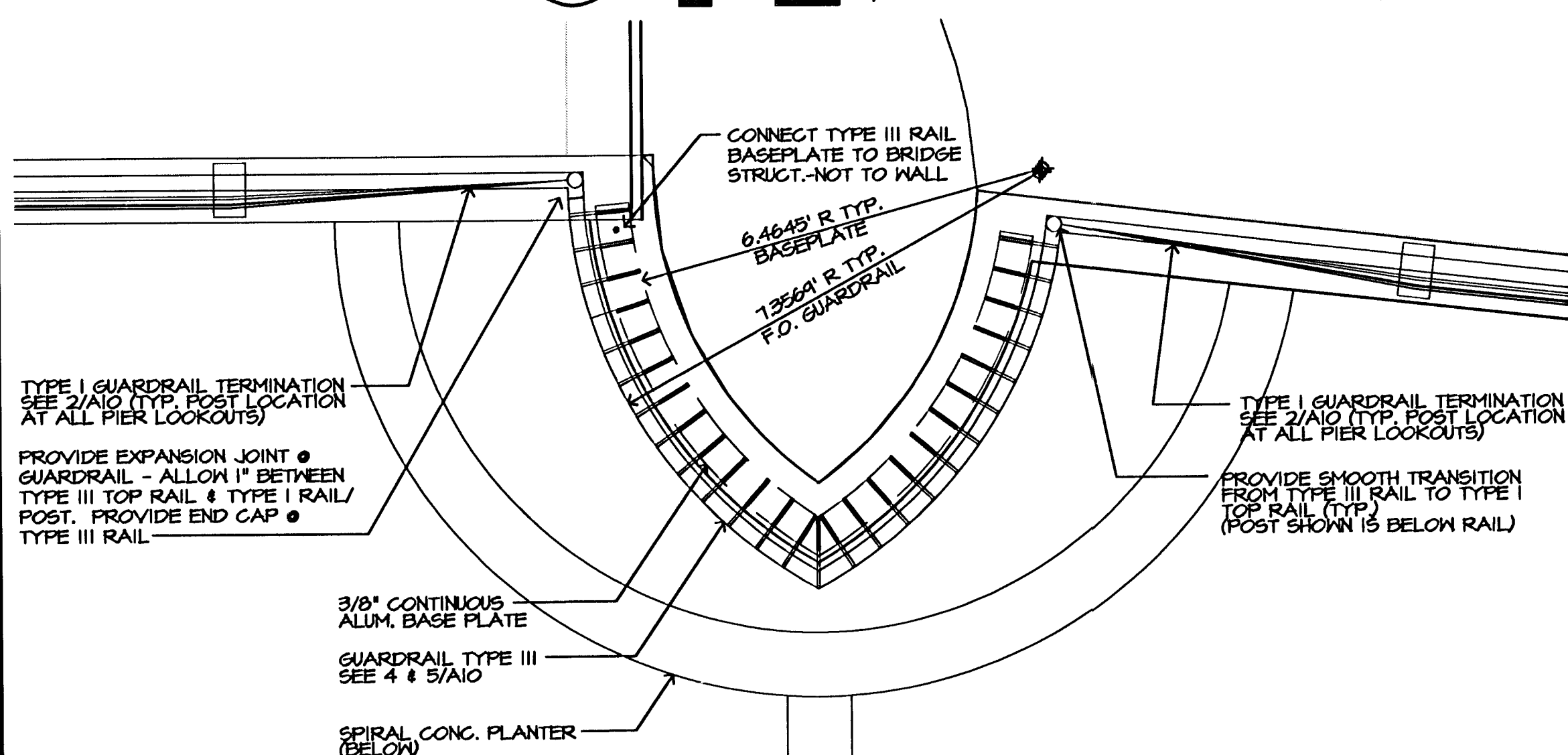
B ENLARGED GUARDRAIL PLAN ABUTMENT LOCATIONS 0' 1' 2' 3' 1/2"=1'-0"
